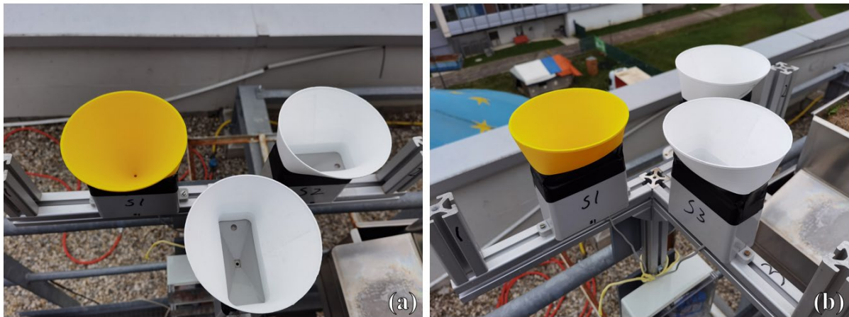
Figure 5-40. New test setups: new additional enlarged funnel in conical shape in yellow color installed on low-cost TBRG No.4 and old additional enlarged funnel in white color installed on low-cost TBRG No.5 and No.6. (a) Top view, (b) Side view.
