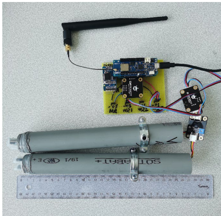
Figure 6. Low-cost water turbidity monitoring station initial setup (no screen at first): antenna on the top, main board in the middle, DFRobot interface circuit on the right, DIY sensor probe on the bottom.
