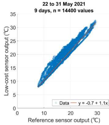
Figure 4-24. BME280 and reference sensor air temperature measurements comparison in May 2021. The correlation function has been selected from the regression results given in Table 4-14.
