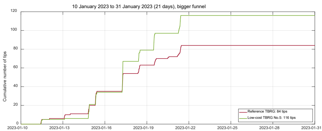
Figure 36. Low-cost TBRG No.5 performance from 10 to 31 January 2023.
