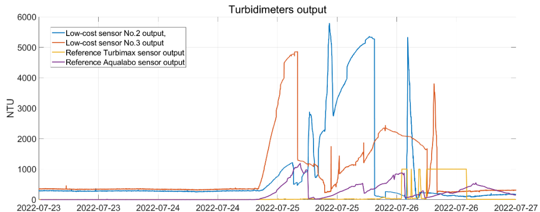
Figure 17. Turbidimeters output at the beginning of the final installation setup
