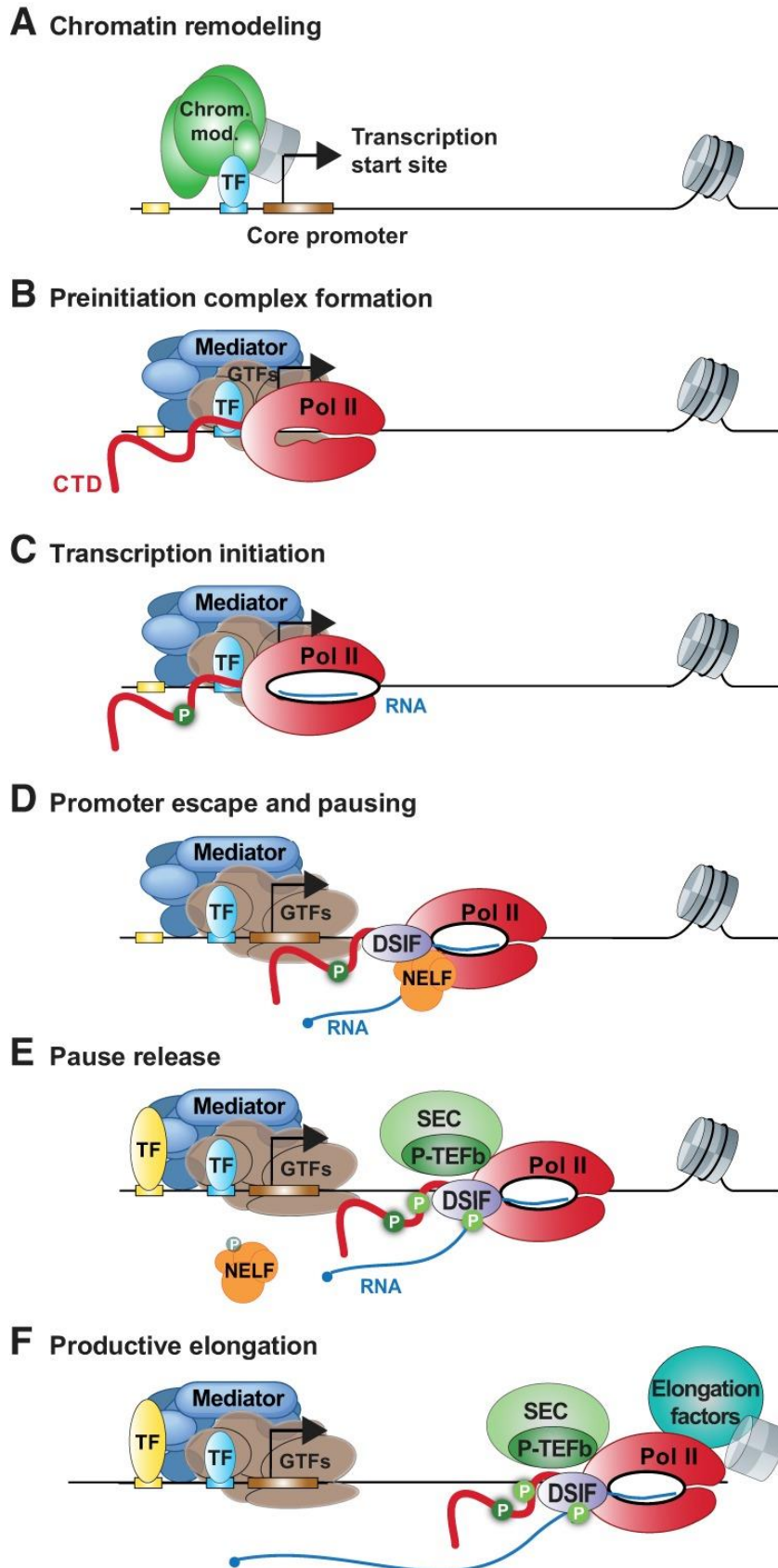
Figure 81. Transcription initiation, RNAPII pausing, and elongation.
