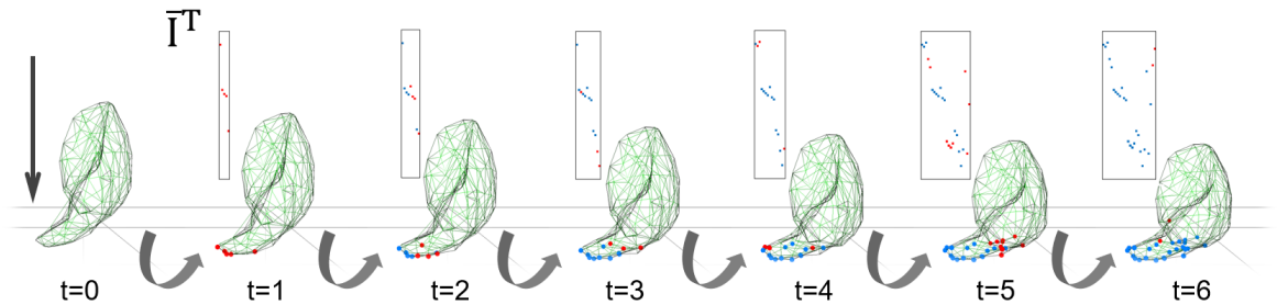
Figure 4.7: The evolution of contact space in a contact simulation between a deformable liver mesh and a rigid plane: The points on the mesh show the isolated DOFs that appear in the previous time steps (blue) and the new isodofs (red). It is revealed that the consecutive time steps usually shares same isodofs , which is relected on the isodof Jacobian matrix \bar{\mathbf{I}} .
