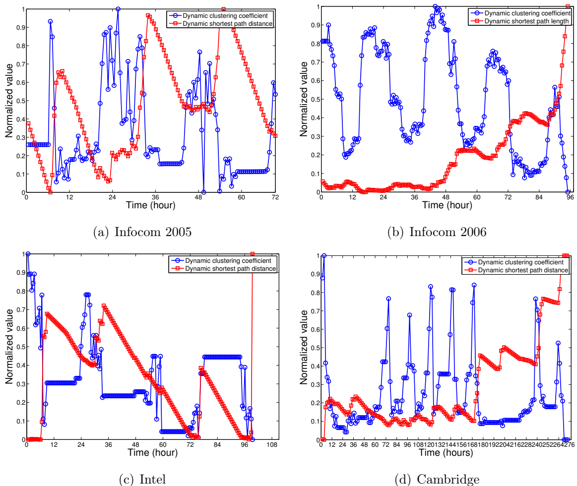
Figure 3.2: Small world phenomenon observed in real mobility traces
