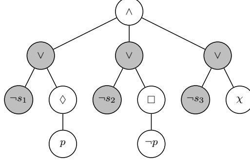
Figure 7.3 – The formula \varphi = (\diamond p \wedge \square \neg p \wedge \chi) with selectors
