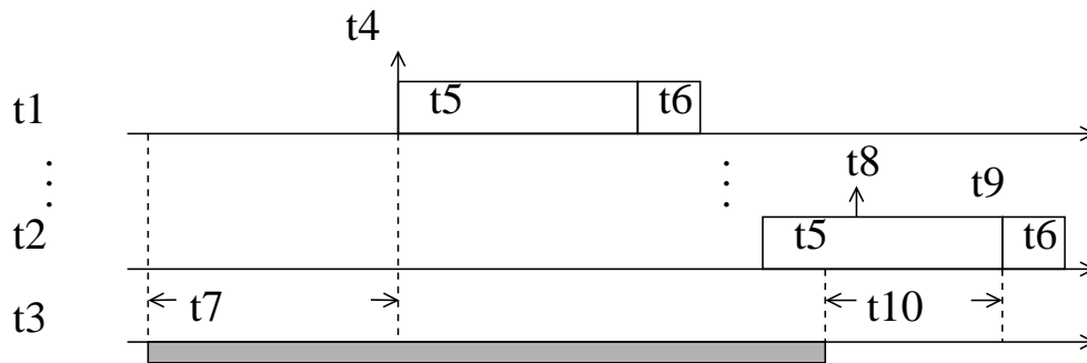
Figure 6.8: Interval of flow with higher priority
