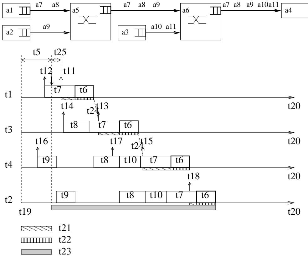
Figure 1.5: Illustration of end-to-end delay of flow \tau_1
