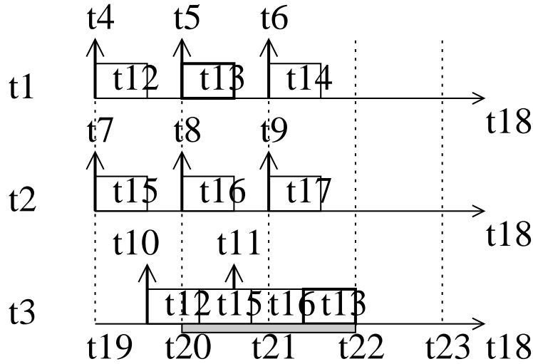
Figure 4.15: Illustration of SingleAssign with increased workload
