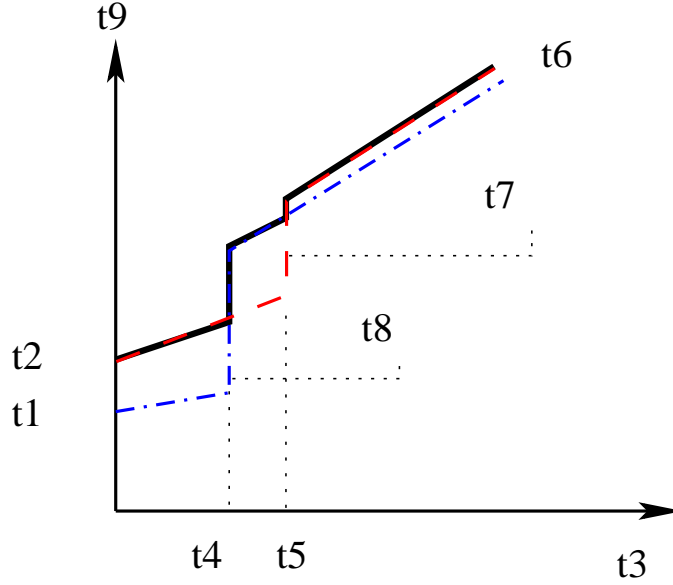
Figure 2.11: The Safe Arrival Curve of subset \mathcal{G}_x
