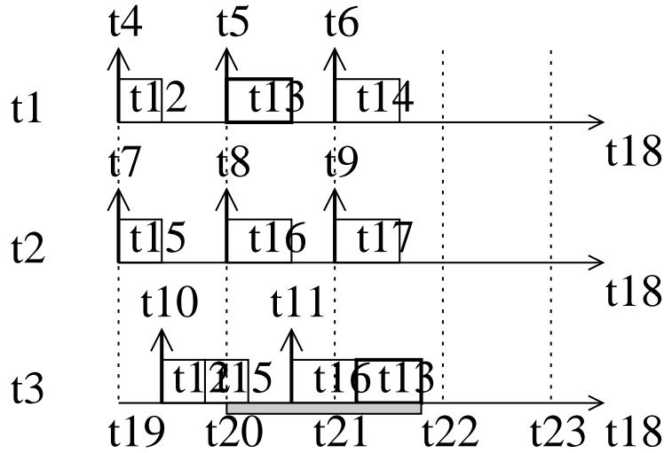
Figure 4.14: Illustration of the SingleAssign with low workload
