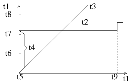
Figure 3.15: Modified approach
