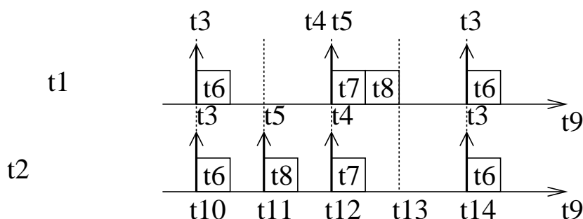
Figure 4.18: Comparison of GCD and SingleAssign
