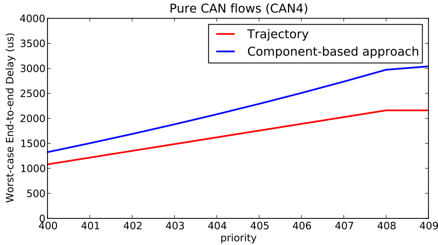
Figure 6.12: Worst-case ETE delay of pure CAN flows
