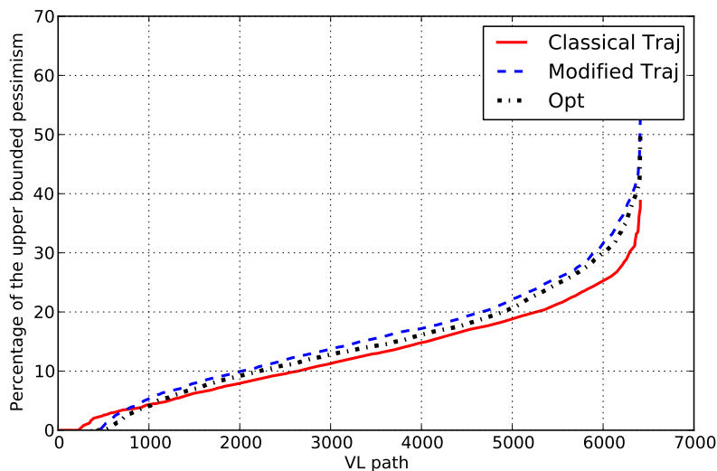
Figure 5.22: Upper bounded pessimism of the Trajectory approach
