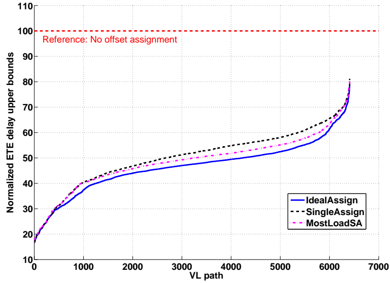
Figure 4.19: Comparative results of IdealAssign , SingleAssign and MostLoadSA
