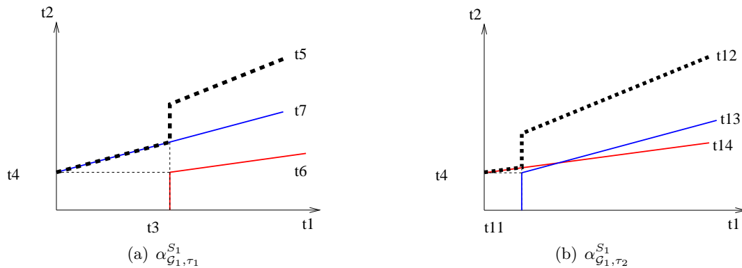
Figure 2.15: Sum arrival curves of \mathcal{G}_1
