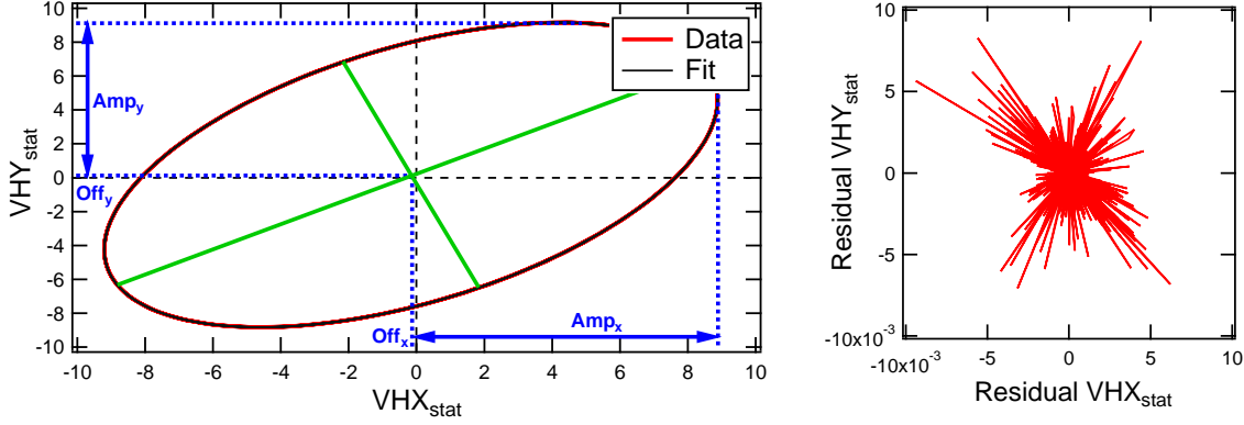
Figure 3.17 On the left, fitting of V_{HY}^{\text{stat}} as a function of V_{HX}^{\text{stat}} with an ellipse to calibrate the parameters of offset, amplitude and the phase shift. On the right, residuals associated to the fit.
