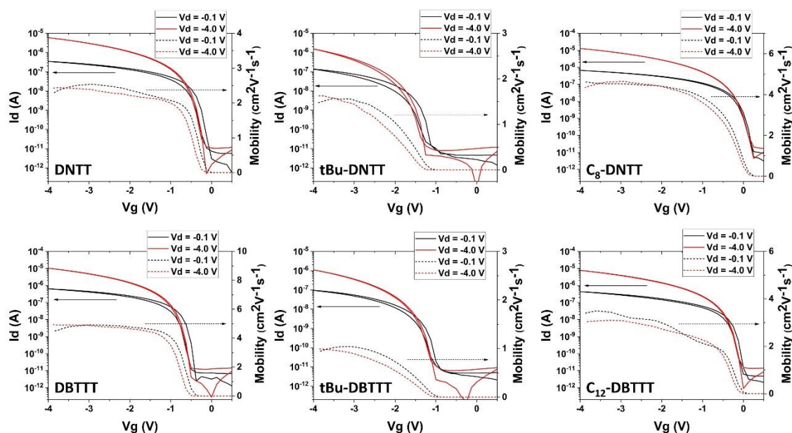
Figure 3.5: Transfer characteristics of BC TFTs with 25-nm-thick OSC layer. Solid lines and dashed lines are referred to drain current and mobility respectively. All TFTs have W/L = 480/215 \mu\text{m} .
