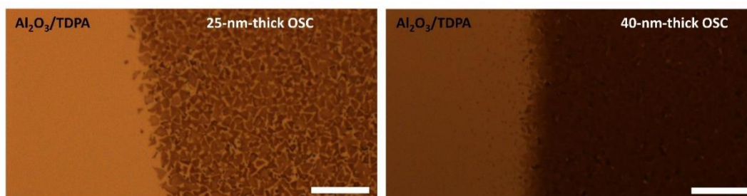
Figure A1.5: Optical micrographs of 25-nm-thick (on the left) and 40-nm-thick (on the right) layer of tBu-BTBT deposited onto \text{Al}_2\text{O}_3/\text{TDPA} at substrate temperature of 70 \text{ }^\circ\text{C} . Scale bar = 20 \mu\text{m} .
