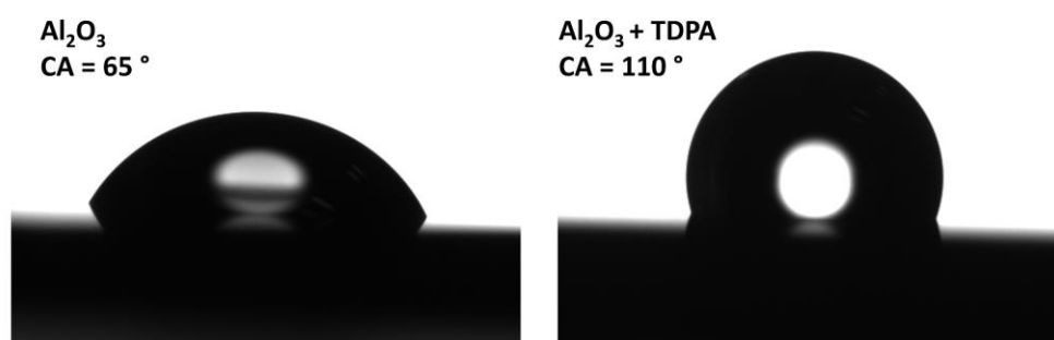
Figure 2.3: Contact angle of water droplets on bare Al 2 O 3 and on TDPA/Al 2 O 3 .
