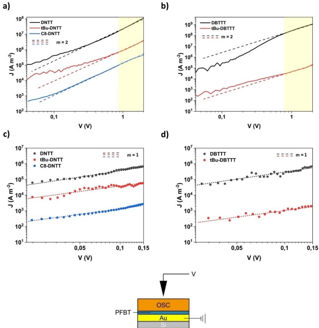
Figure 3.18: J-V characteristics measured using C-AFM on thin films plotted in logarithmic scale.
