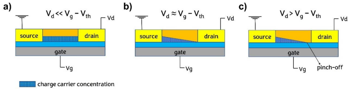
Figure 1.7: Charge carrier concentration profile of OFETs. (a) linear regime, (b) starting point of saturation regime and (c) full saturation regime.
