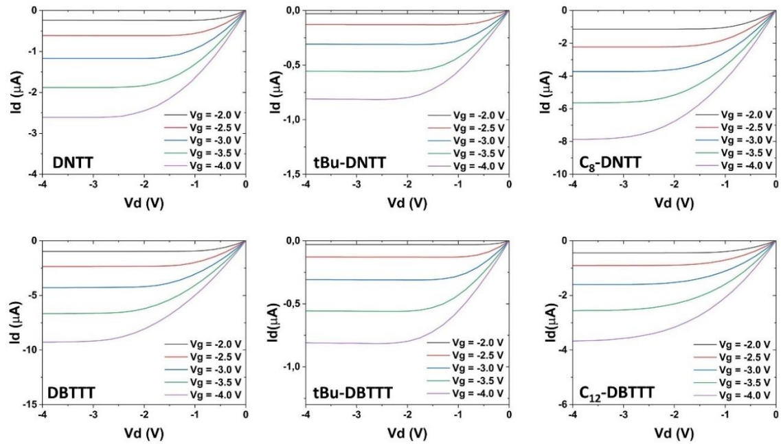
Figure A2.1: Output characteristics of TC TFTs with 25-nm-thick OSC layer. All TFTs have W/L = 480/215 μm.
