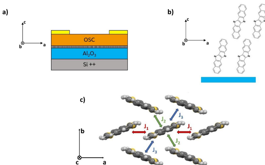
Figure 2.22: Molecular arrangement with respect to a , b and c directions. a) schematic illustration of a TFT with the active layer along the ab plane. (b) Example of the molecular arrangement of DN4T onto the dielectric (in light blue), with the molecules standing approximately upright with respect to the substrate. (c) Schematic illustration of transfer integrals within adjacent molecules along the ab plane.
