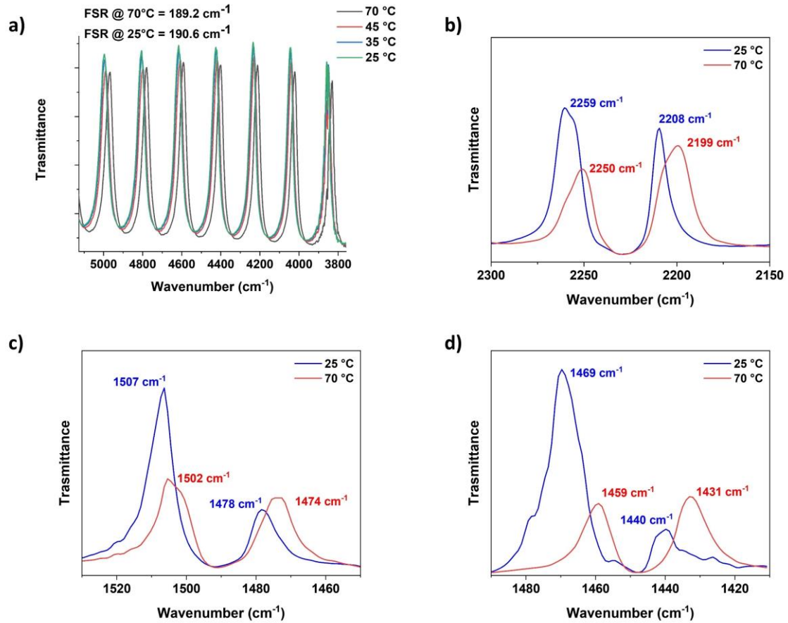
Figure 4.7: Shift of the optical cavity modes due to temperature change. (a) Evolution of the optical cavity modes of an empty FP cavity when cooled from 70 °C to 25 °C. (b),(c) Shifts of the polaritonic states obtained in VSC1, referring to the coupling between the benzonitrile vibration at 2228 cm -1 and the 18 th optical mode and to the cooperative VSC between the vibration at 1492 cm -1 and the 12 th optical mode. (d) Shifts of the polaritonic states obtained in VSC2, referring to the coupling between the benzonitrile vibration at 1445 cm -1 and the 12 th optical mode
