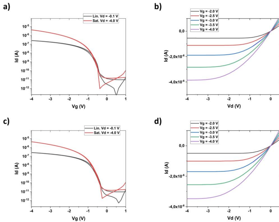
Figure A1.1: Transfer and output characteristics of C_8 -DN4T and C_{10} -DN4T TC devices. On the top: representative transfer (on the left) and output (on the right) characteristics of BC TFTs based on (a),(b) C_8 -DN4T and (c),(d) C_{10} -DN4T at substrate temperature of 100 °C. TFTs have W/L = 480/215 \mu\text{m} .
