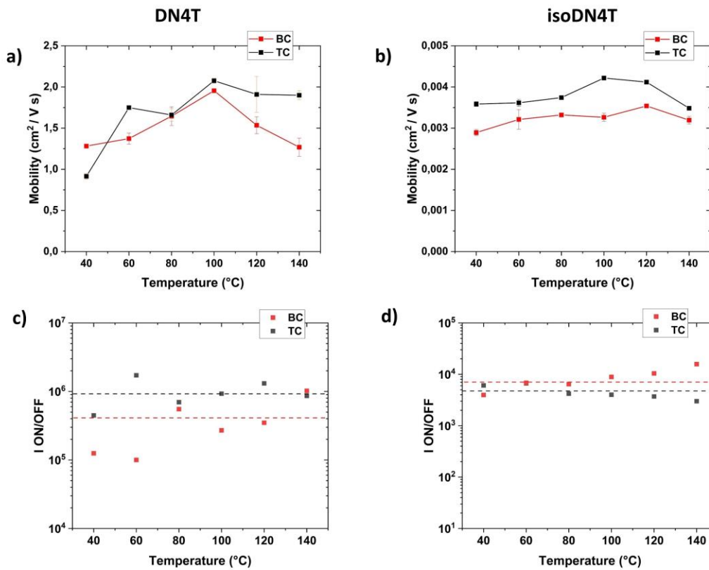
Figure 2.13: Mobility and on/off current ratio vs substrate temperature for BC and TC TFTs based on DN4T and isoDN4T.
