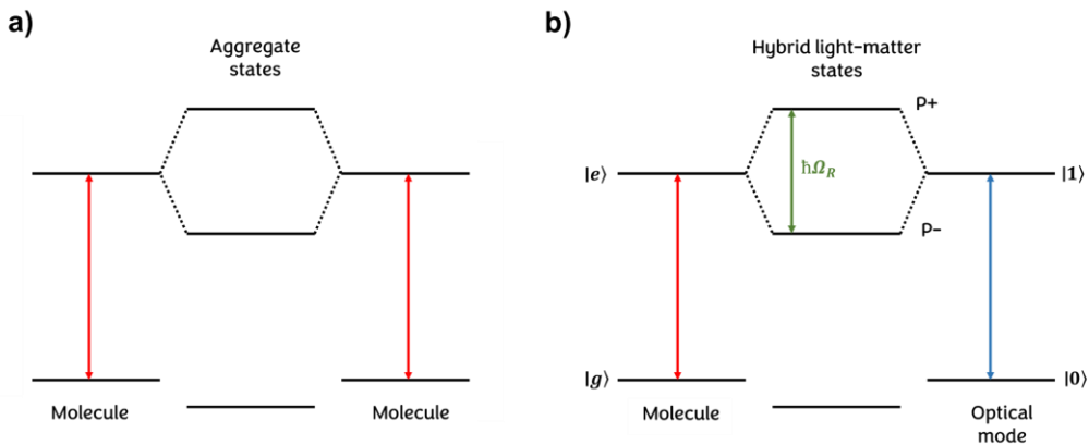
Figure 1.15: Schematic energy diagrams of light-matter interaction. Schematic illustration of (a) the electronic coupling between transition dipole moments resulting in the formation of J- and H-aggregates and (b) the analogy with the interaction between a molecular transition and an optical mode resulting in the formation of two new hybrid light-matter states ( P^+ and P^- ).
