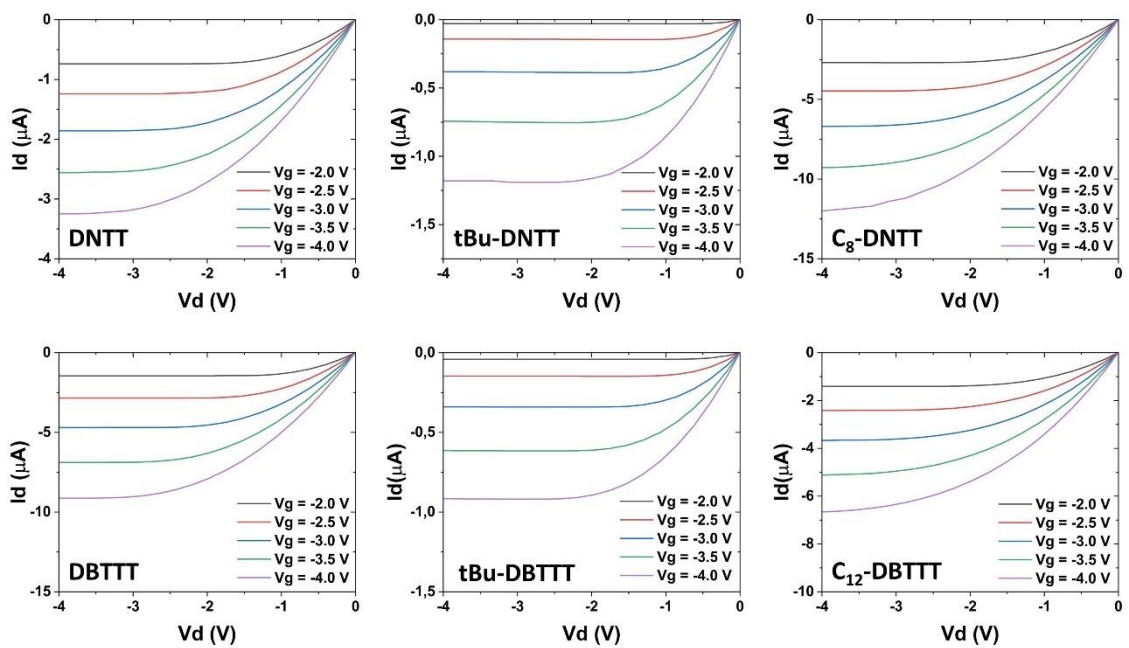
Figure A2.2: Output characteristics of BC TFTs with 25-nm-thick OSC layer. All TFTs have W/L = 480/215 μm.
