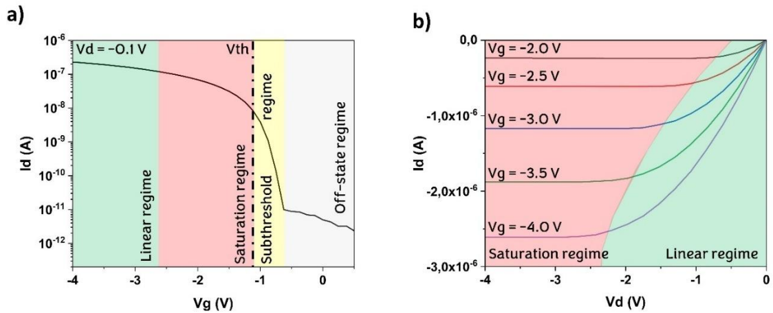
Figure 1.8: Transfer and output characteristics of a p-type OFET. (a) Transfer and (b) output characteristics. Depending on the values of V_g and V_d , the different regimes of operations are highlighted.
