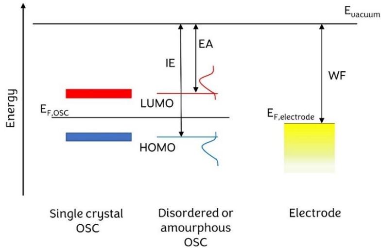
Figure 1.3: Organic semiconductor and electrode energy band diagrams. Schematic illustration of (a) single crystal OSC where narrow conduction (in red) and valence (in blue) bands are formed, (b) disordered or amorphous OSC where distribution of states are formed and (c) metal electrode.
