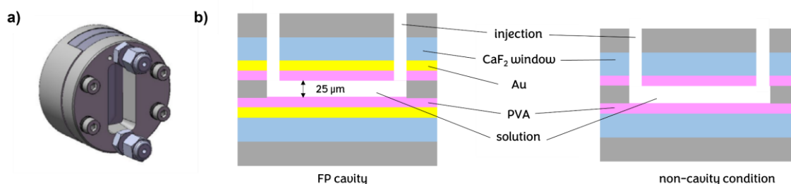
Figure 4.4: Fabry-Perot cavity.
