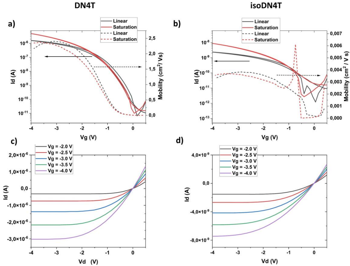
Figure 2.15: Transfer and output characteristics of DN4T and isoDN4T bottom-contact devices.
