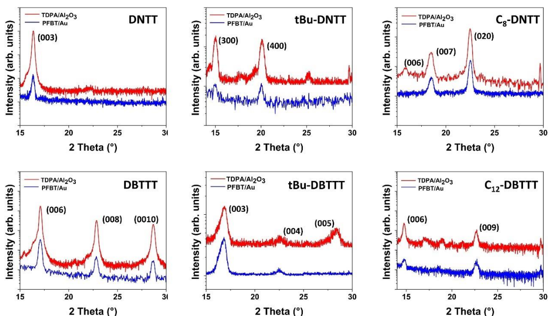
Figure 3.3: XRD patterns of OSCs deposited onto TDPA/Al 2 O 3 and PFBT/Au substrates. The thin films have nominal thickness of 25 nm.
