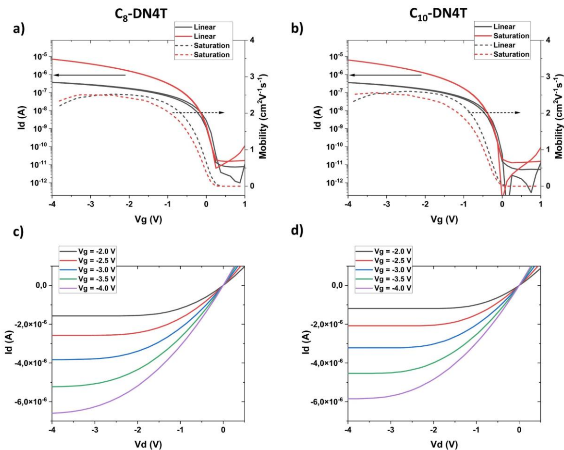
Figure 2.17: Transfer and output characteristics of C 8 -DN4T and C 10 -DN4T bottom-contact devices.
