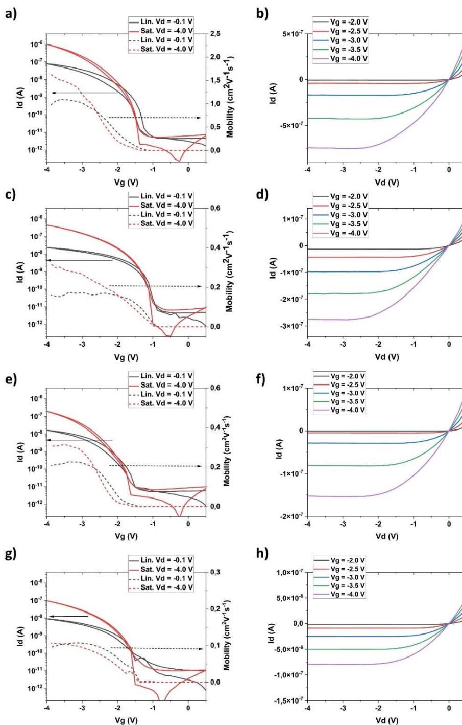
Figure A1.3: Transfer (left) and output (right) characteristics of the best performing TC TFTs based on tert -butyl theienoacene derivatives. (a, b) tBu-DNTT , (c, d) tBu-DBTT , (e, f) tBu-BTBT-1 and (g, h) tBu-BTBT-2 . In transfer characteristics, solid lines and dashed lines are referred to drain current and mobility respectively. All TFTs have W/L = 480/215 \mu\text{m} .
