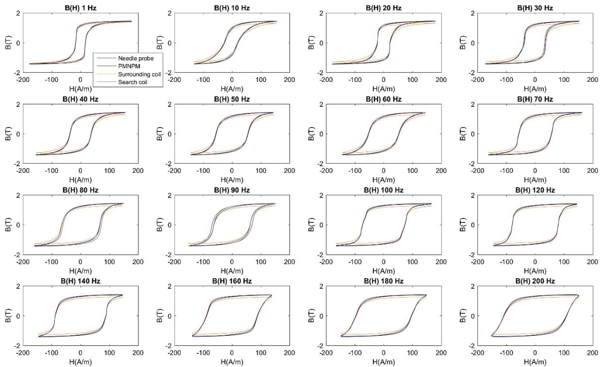
Figure 4-1: Frequental B H characteristic curves of RD-GO steel sheet as seen by 4 sensor( classic needle probe, 10 turns surrounding coil, search coil and PMNP)
