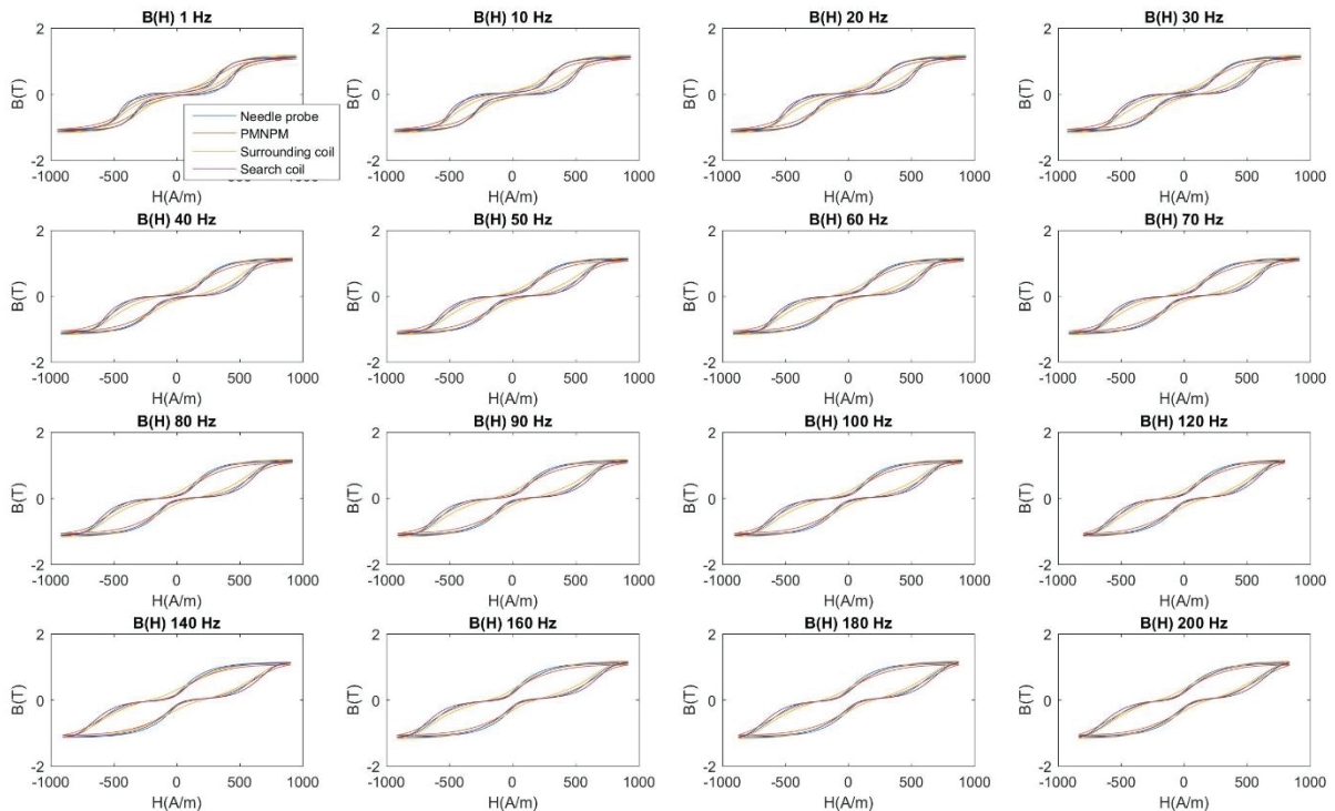
Figure 4-2: Frequental B H characteristic curves of TD-GO steel sheet as seen by 4 sensors( classic needle probe, 10 turns surrounding coil, search coil and PMNP)
