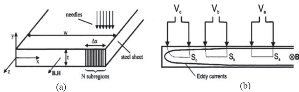
Figure 2-3 : (a) Needle probe method ; (b) Eddy-current distribution in a sample surface and edges [74]
