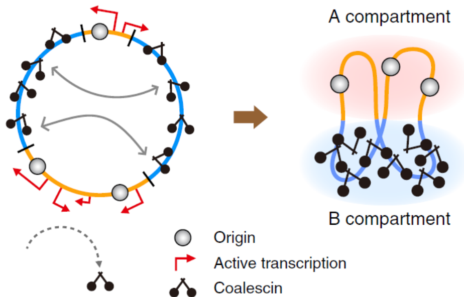
Figure 12: Chromosome organization in Sulfolobus
