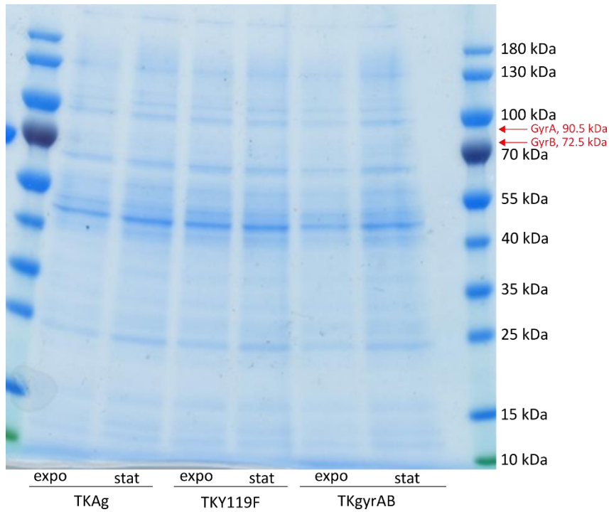
Supplementary figure 2. SDS-PAGE analysis of soluble proteins from T. kodakarensis .
