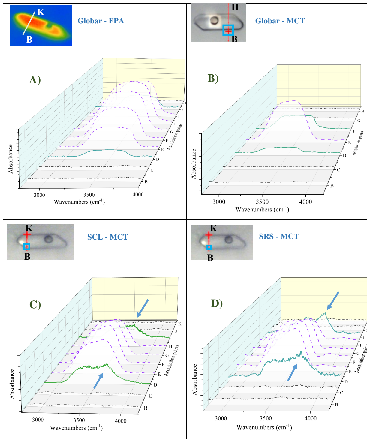
Figure 4.9. The variation of OH stretching band recorded across the SFI-1 before processing steps (from point B to point H or K) with A) Globar source with FPA detector (aperture-less microscope), B) Globar source with MCT detector, C) supercontinuum laser with MCT detector, and D) synchrotron beam with MCT detector. Black lines (dash-dot line) correspond to quartz, green (solid line) to the near liquid-solid interface, and purple (dash line) to bulk water behavior. The blue squares in panels B, C, and D correspond to the aperture size.
