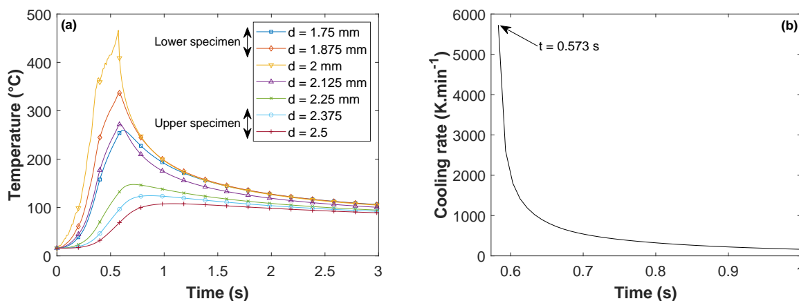
Figure 4.22: Temperature evolution at different location through the interface (a) and cooling rate evolution at the interface (b)
