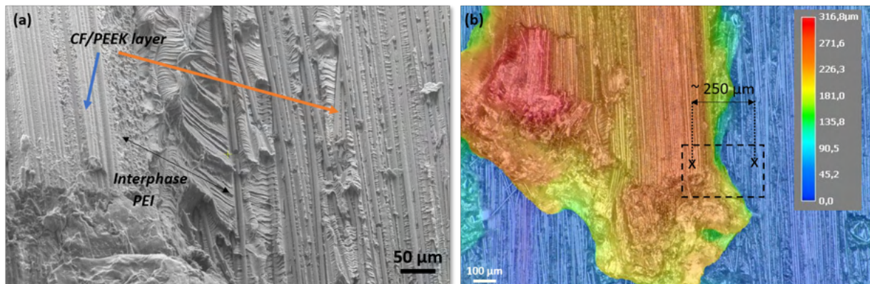
Figure 5.15: SEM (a) and optical (b) micrographs of interfacial fracture between two layers of CF/PEEK, color chart corresponds to a difference in height
