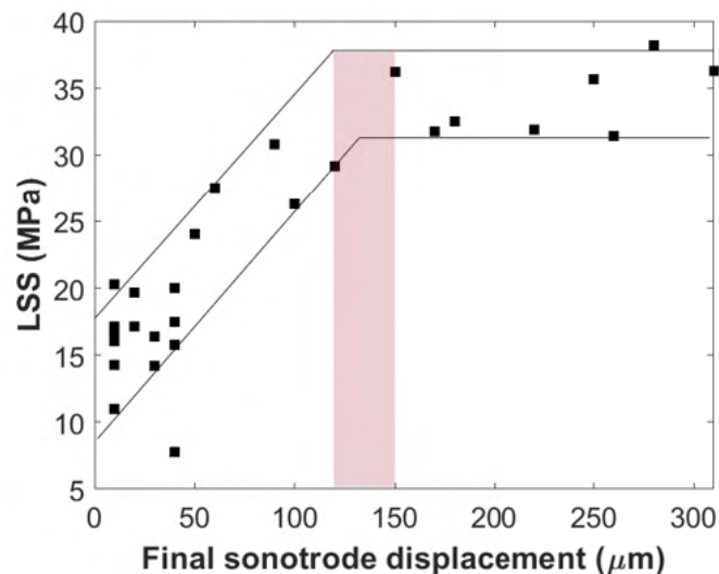
Figure 5.33: Final sonotrode displacements for AE 250 specimens in configuration B
