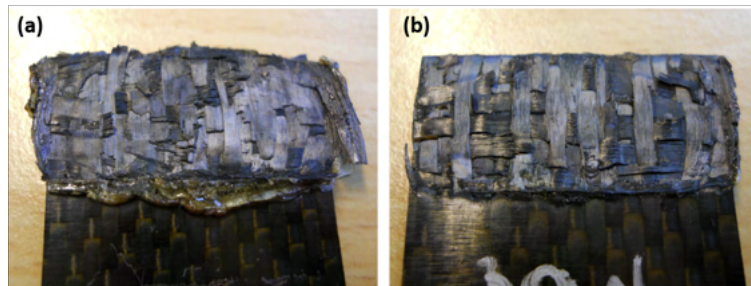
Figure 1.17: Interfacial fracture of CF/PEI welds at 300 N load and 86.2 \mu\text{m} amplitude (a) and 300 N load and 51.8 \mu\text{m} amplitude (b) [Villegas, 2014]
