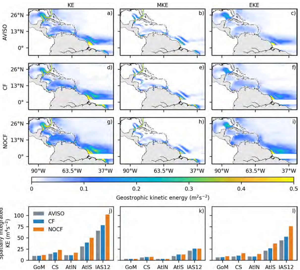
Figure 3.3: KE (first column), MKE (second column), and EKE (third column) climatologies over the IAS for AVISO (first row), CF (second row), and NOCF (third row). j–l) Spatially integrated energy over the regions comprising the IAS is shown in the bottom row.
