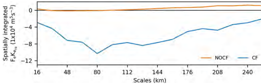
Figure 6.1: Geostrophic eddy wind work F_e K_{e_{cg}} for scales ranging from 16 km to 256 km and spatially integrated over the polygon delimited by the black segmented contours in Figure 6.2 and out of the shelf delimited by the 200 m depth contour.
