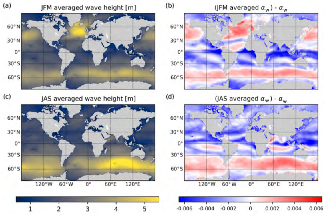
Figure 1.27: Mean differences in the wind stress computed with and without the influence of surface waves over 3-year numerical simulations. The figure is taken from Couvelard et al. (2020).
