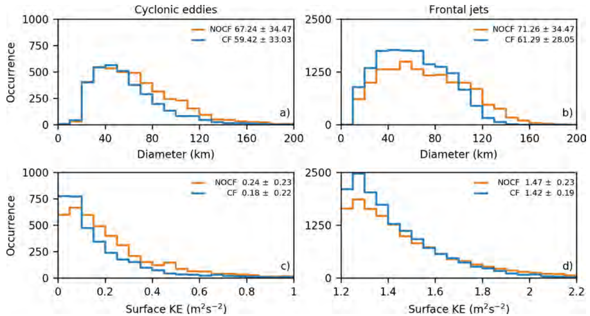
Figure 6.4: 24-year statistics about the diameter (first row) and KE (second row) of cyclonic eddies (first column) and frontal jets (second column). The mean and standard deviation of cyclonic eddies and frontal jets properties are included on the top right corner.
