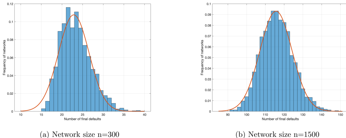
Figure 2.2: Histograms of 3000 times Monte-Carlo simulation for the number of final defaults in regular financial networks with size n = 300, 1500 .
