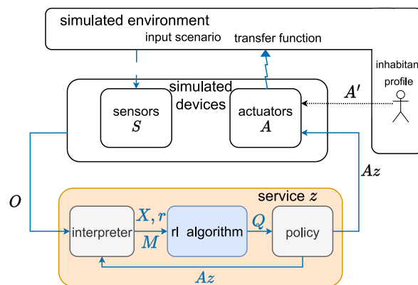
FIGURE 5.7 – Simulated RL-based simple smart home system
