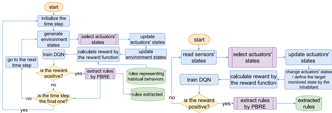
FIGURE 7.10 – Rule extraction without "refining rules" in a smart home system with one service in simulation FIGURE 7.11 – Rule extraction without "refining rules" in a smart home system with one service in the real world
