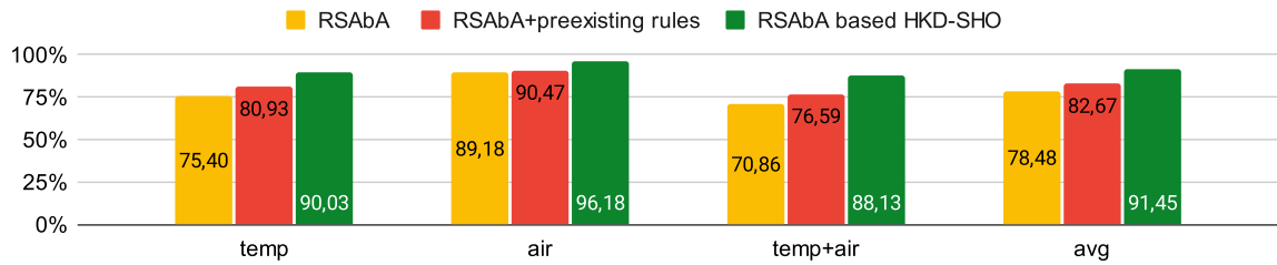
FIGURE 8.3 – Evaluation results with RSAbA being the machine learning-based system and without constraint in the inhabitant’s profile
