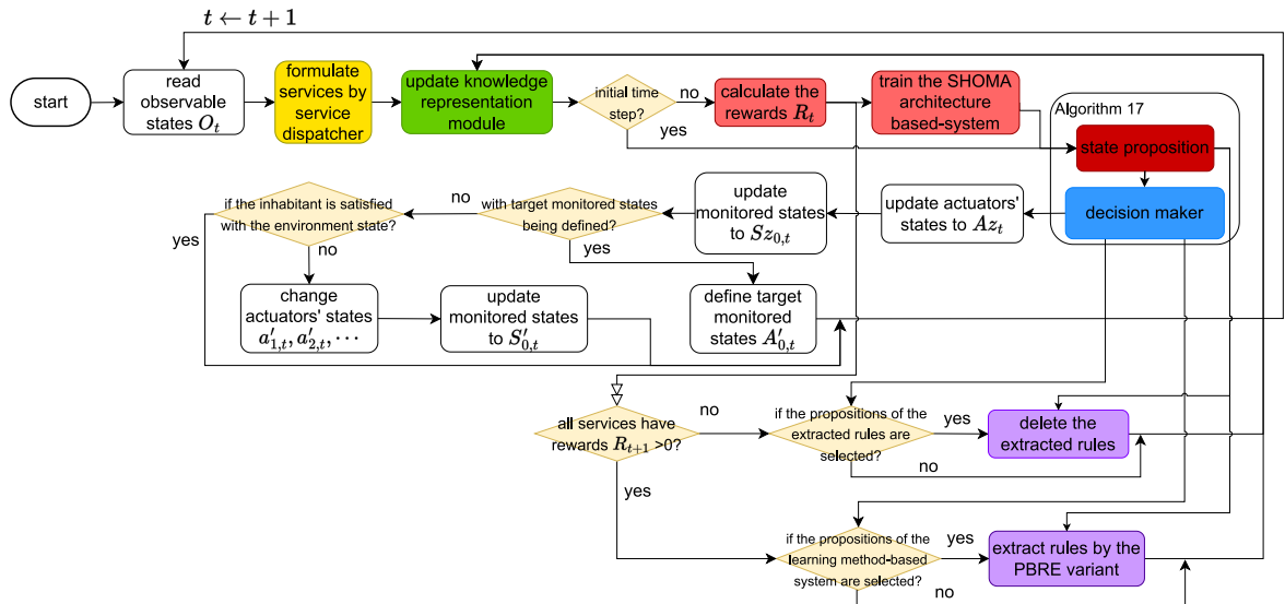
FIGURE 8.2 – Detailed working process of HKD-SHO
