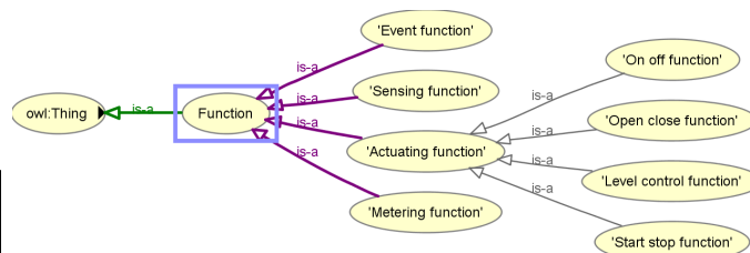
FIGURE 2.7 – SubClasses of class "Function"
