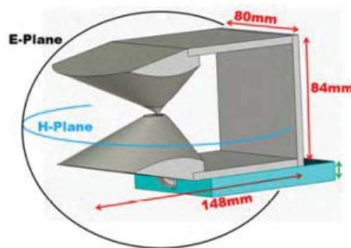
Figure 17 : Antenne Shark [52]
