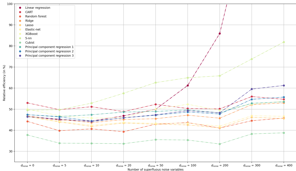
Figure 5: Relative efficiency of model-assisted estimators \hat{\tau}_{ma}^{(j)} , j = 1, \dots, 12 for the estimation of the total of Y_2 with SRSWOR, n = 600 and increasing number of auxiliary variables
