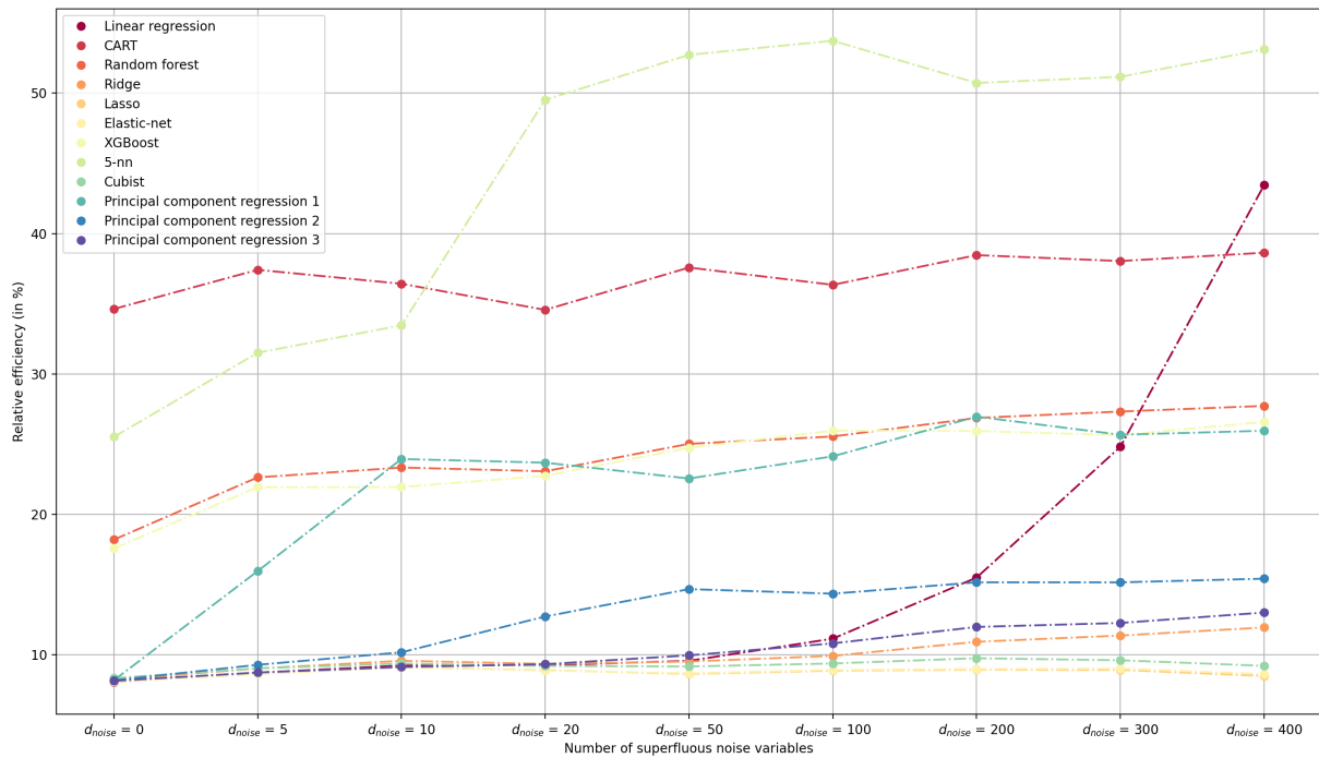
Figure 4: Relative efficiency of model-assisted estimators \hat{\tau}_{ma}^{(j)} , j = 1, \dots, 12 for the estimation of the total of Y_1 with SRSWOR ( n = 600 ) and increasing number of auxiliary variables
