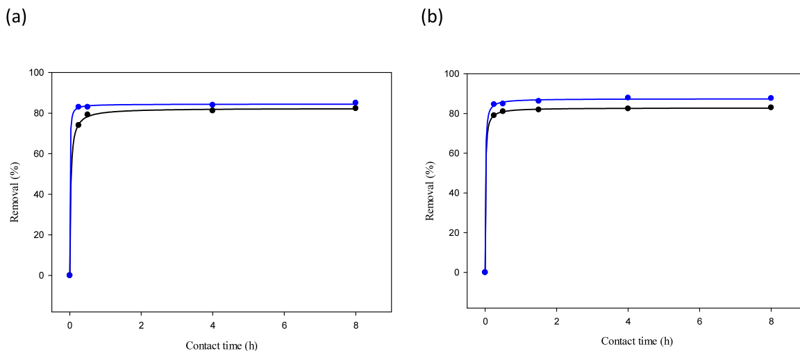
Fig. 2. Effect of contact time on difenoconazole adsorption (in %) on Douce Terre (DTP, blue curve) and Champ Marie (CMP, black curve) soils (conditions: volume 50 mL; soil 10 g; temperature 25 °C; n = 3 ; difenoconazole concentration C_0 1 mg L -1 (a) and 15 mg L -1 (b)). (For interpretation of the references to color in this figure legend, the reader is referred to the web version of this article.)
