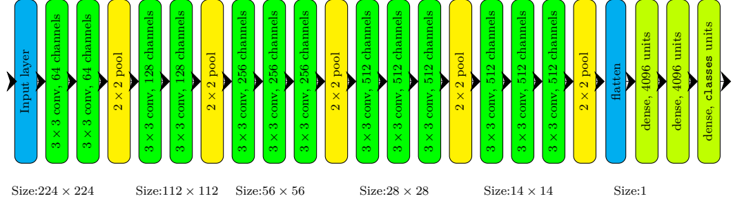
Figure 1.8: Architecture of the VGG-16 network for an input image of size 224 × 224.
