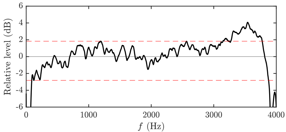
Figure 2.6 – Frequency response measured in the axis of the loudspeaker designed for the propagation study. Dashed lines indicate the minimum and maximum levels in the frequency band [90 - 3150] Hz.
