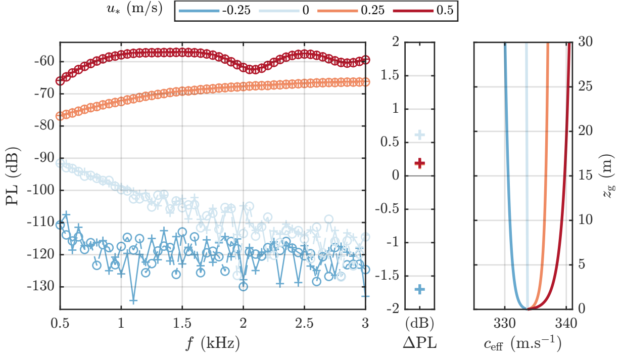
Figure 6.7 – PL spectrum in several wind conditions for reciprocal (solid line, +) and direct (dashed line, o) pressure field computation (left), overall \Delta\text{PL} weighted according to the ptarmigan spectrum (middle), and c_{\text{eff}} profiles associated (right). Refraction conditions are defined by u_* varying from -0.25 to 0.5 m/s, while \theta_* = 0 K.
