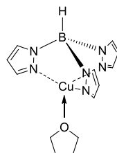
Figure 19: Hydrotris(pyrazol-1-yl)-borato]cuivre(I) adduit THF, [\text{CuTp}^{\text{H}}] .
