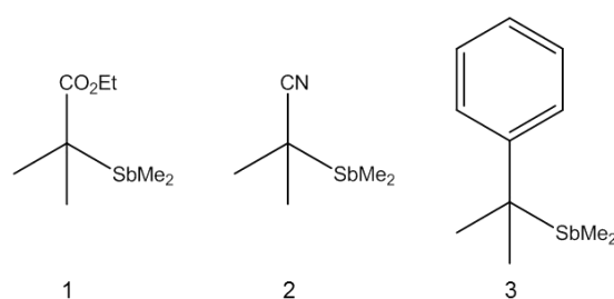
Figure 31: Organostibines used in reference 169 to control the polymerization of NVP.
