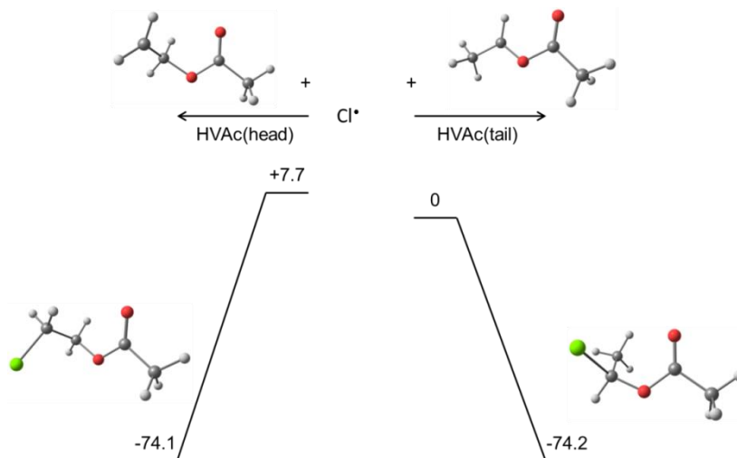
Figure 99: Relative BPW91* enthalpies (in kcal/mol) and optimized geometries of the species implicated in the deactivation process of the T and H PVAc radical models by ATRP ( X = \text{Cl}^\bullet ).
