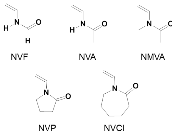
Figure 91: Structure of the five unconjugated N -vinyl amides studied by Debuigne and coworkers (NVF = N -vinyl formamide, NVA = N -vinyl amide, NMVA = N -methyl- N -vinyl acetamide, NVP = N -vinyl pyrrolidone, NVCl = N -vinyl caprolactam).
