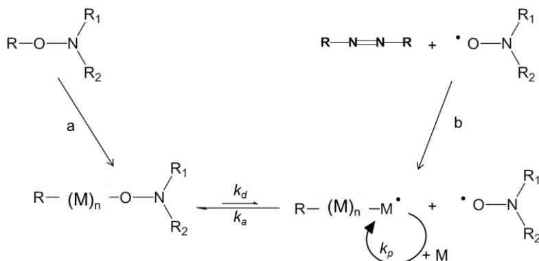
Scheme 3: Activation-deactivation equilibrium in NMP. Monocomponent (a) and bicomponent (b) initiating system.
