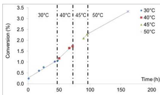
Figure 72: Conversion of vinyl acetate vs. time (conditions: 30-50°C, [\text{Cu}(\text{NacNac}^{\text{XylXyl}})(\text{MeCN})] / \text{VAc} / \text{V-70} = 1 : 500 : 0.7 ; \text{VAc}/\text{toluene} = 15:85 v/v).
