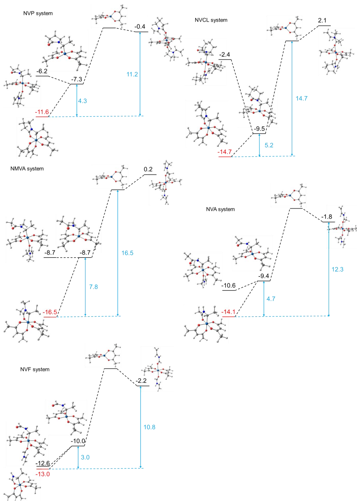
Figure 96: Relative enthalpies in kcal/mol and views of the optimized geometries of the monomer addition products to K^1\text{:C}[\text{Co}(\text{acac})_2(\text{MH})] and [\text{Co}(\text{acac})_2] . For comparison, the K^2\text{:C,O}[\text{Co}(\text{acac})_2(\text{MH})] system is also shown.
