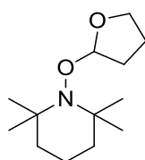
Figure 85: TEMPO-THF adduct.
