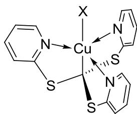
Figure 55: Structure of [\text{Cu}(\text{TPTM})\text{X}] reported by Kinoshita in reference 230 ( \text{X} = \text{F}, \text{Cl}, \text{Br}, \text{I} ).
