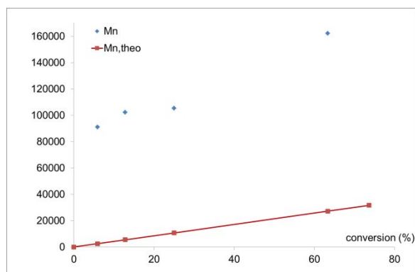
Figure 74: PVAc molecular weights evolution with VAc conversion ( [\text{Cu}(\text{Tp}^{\text{CF}_3})(\text{MeCN})] / \text{VAc} / \text{V-70} = 1 : 500 : 0.8 in bulk) (Blue dots). Theoretical molecular weights (red line).
