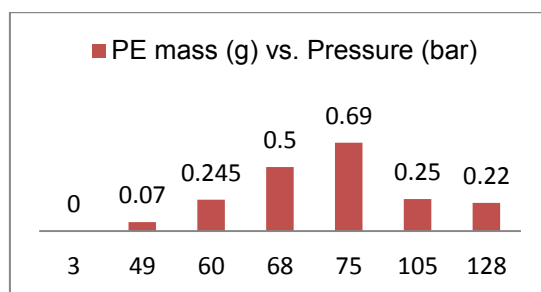
Figure 87: Variation of PE self-production under various ethylene pressure (conditions: THF / ethylene, T = 90^{\circ}\text{C} ).
