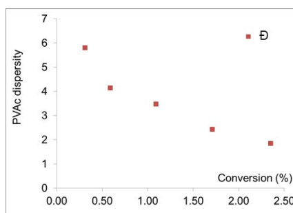
Figure 78: Dispersity evolution of PVAc obtained from polymerization [CuTp^*]_2 in diluted medium (30°C, [CuTp^*]_2 / VAc / V-70 / \text{toluene} = 0.5 : 500 : 0.7 : 80\%v ).
