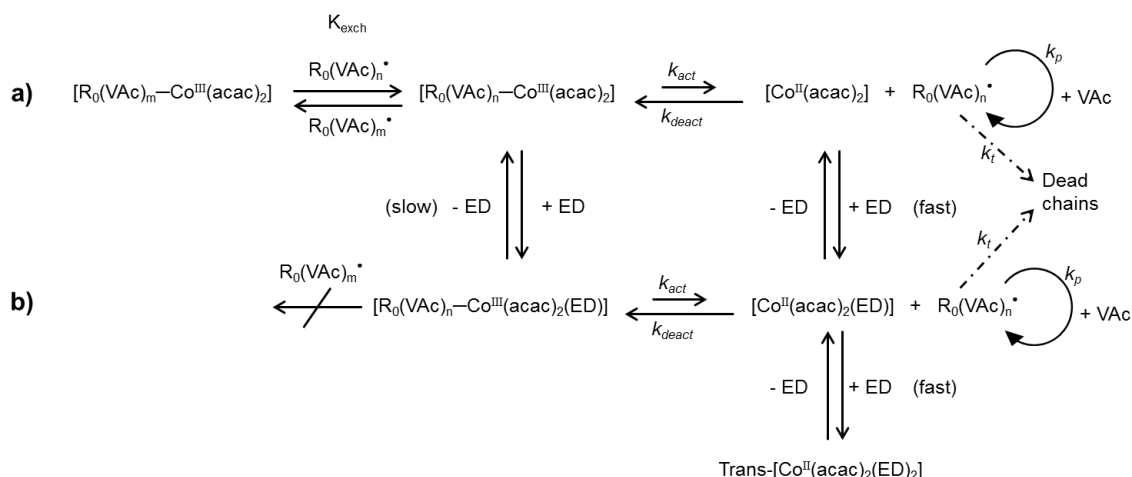
Scheme 16: Proposed general mechanism for the CMRP of VAc mediated by [\text{Co}(\text{acac})_2] complex in the a) absence and b) presence of EDs.
