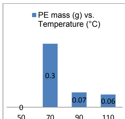
Figure 88: Variation of PE self-production under various temperature (conditions: THF / ethylene, P = 51 \pm 2 bars).
