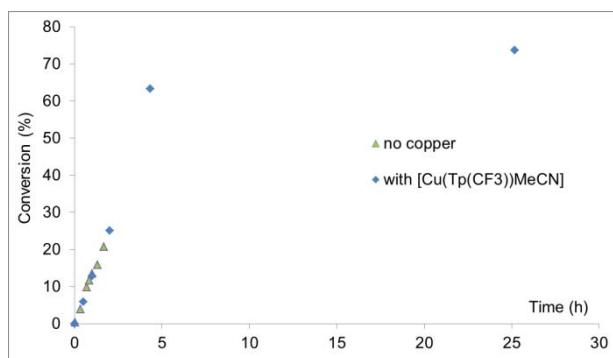
Figure 75: Kinetic profile of VAc polymerizations with [\text{Cu}(\text{Tp}^{\text{CF}_3})(\text{MeCN})] and without copper ( [\text{Cu}] / \text{VAc} / \text{V-70} = 1 : 500 : 0.8 or \text{VAc} / \text{V-70} = 500 : 0.8 in bulk at 30°C).
