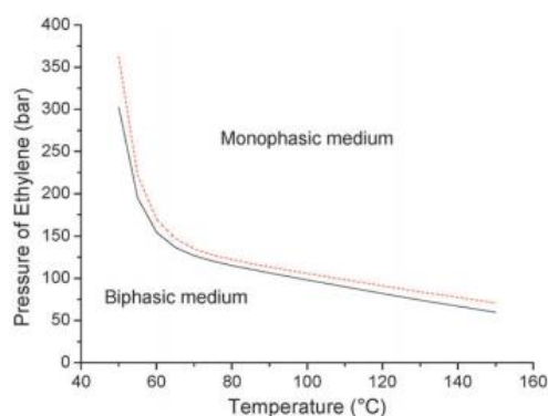
Figure 86: Phase diagram of ethylene/solvent system in a 230 mL reactor with 50 mL THF (black line) and 50 mL toluene (dashed red line) from reference 258.
