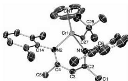
Figure 25: [\text{neopentyl-CpCr}^{\text{III}}(\text{NacNac}^{\text{XylXyl}})] complex used as a single-component OMRP reagent in reference 66.
