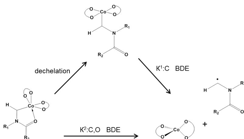
Scheme 26: Dechelation and homolytic bond cleavage processes for the dormant species in [Co(acac) 2 ]-mediated polymerization of vinyl amide monomers (acac = acac).
