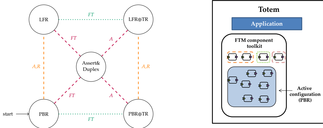
Figure 5.9: Transition Scenario (left) and FTM Component Toolkit Deployed on Totems (right)
