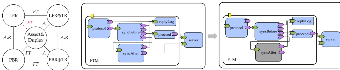
Figure 4.8: LFR→Assert&Duplex Transition: Scenario (left); Initial and Final Component-Based Architectures (center and right)
