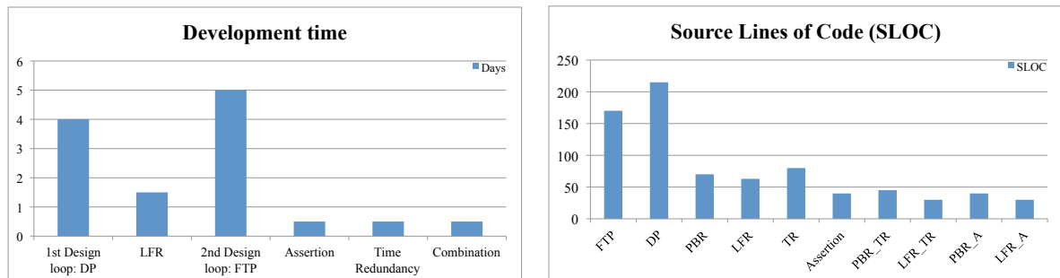
Figure 3.7: FT Toolbox Design and Implementation: Development Time (left) and Source Lines of Code (right)
