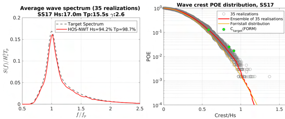
Figure 4.7 – Average wave spectrum of 35 realizations and corresponding wave crest probability distributions, SS17
