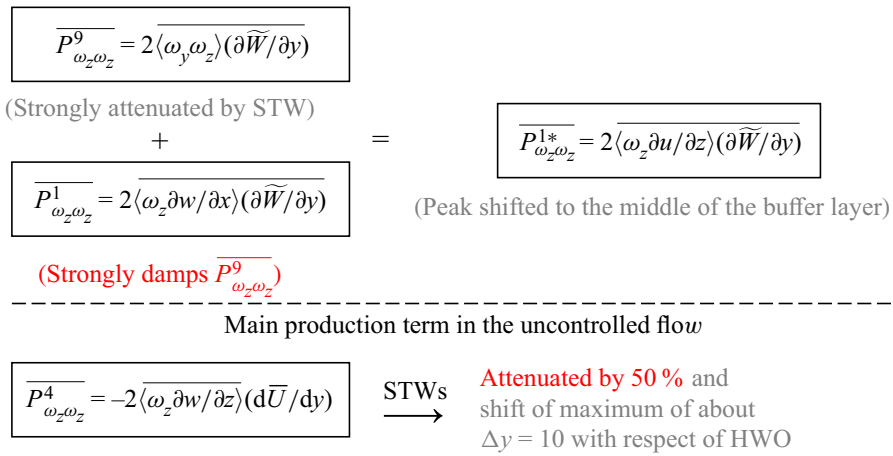
Figure 7. Summary of main characteristics of the effect of control on the spanwise turbulent entrophy production process.
