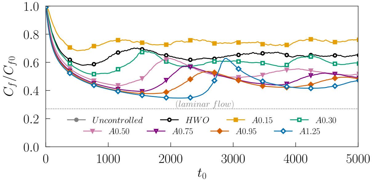
Figure 4.1: Initial response of the normalized skin-friction coefficient ( C_f/C_{f0} ) after the actuation of control for different forcing amplitudes. The long time averaged skin-friction coefficient for the uncontrolled case is C_{f0} = 8.02 \times 10^{-3} .
