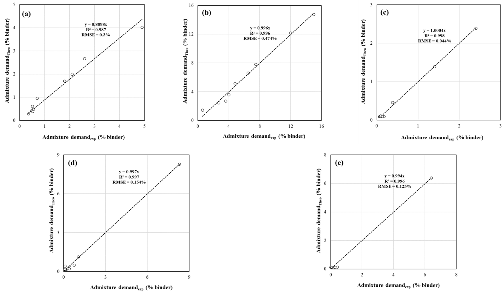
Fig. 4.18. Comparison between the experimental admixture demand and those obtained using the empirical correlations (Eq. 4.4 and Table 4.8) for (a) NaHMP, (b) NaSiI, (c) PCE, (d) PNS, and (e) NE-PC admixtures.
