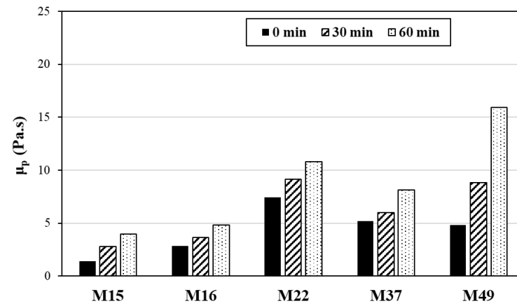
(a) (b) Fig. 6.11. Bingham (a) yield stress and (b) plastic viscosity of the PCE-contained CEM mixtures.
