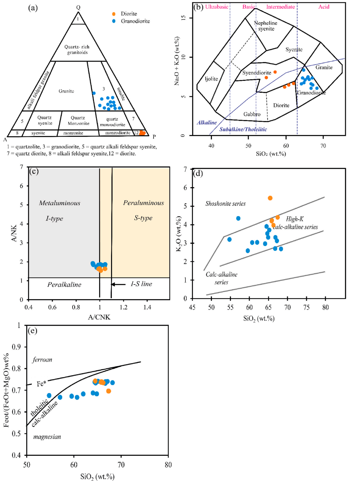
Fig. 4. Major element classification plots of the Deng-Deng granitoids. (a) Modal alkali feldspar (A), quartz (Q), and plagioclase (P) classification of Streckeisen (1976); (b) Total alkalis (Na 2 O+K 2 O wt%) vs. SiO 2 (wt %) classification of plutonic rocks (Cox et al., 1979). (c) Molar [Al 2 O 3 /(CaO+Na 2 O+K 2 O)] versus [Al 2 O 3 /(Na 2 O+K 2 O)] diagram (after Shand, 1951). The samples plot exclusively in the I-type granites field and display metaluminous to slightly peraluminous affinities; (d) K 2 O versus SiO 2 diagram (Peccherillo and Taylor, 1976) showing the plot of the studied granitoids in the high-K calc-alkaline to shoshonitic fields. (e) SiO 2 versus FeOt/(FeOt +MgO) diagram (Frost et al., 2001) depicting the magnesian nature of the Deng-Deng granitoids.
