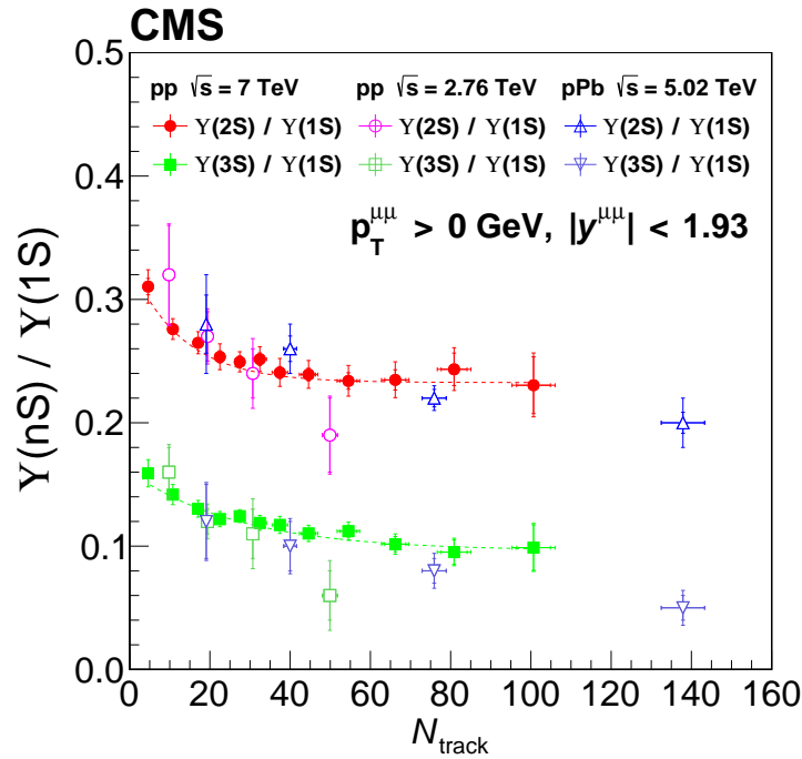
Figure 1.12: The ratios of the Y(2S) -over- Y(1S) and Y(3S) -over- Y(1S) , with p_T > 0 GeV, as a function of the number of tracks ( N_{\text{track}} ) in various collision systems. The lines are fits to the data with an exponential function. The vertical error bars represent the combined statistical and systematic uncertainties on the bottomonia ratio, while the horizontal error bars represent the uncertainty on N_{\text{track}} [61, 62].
