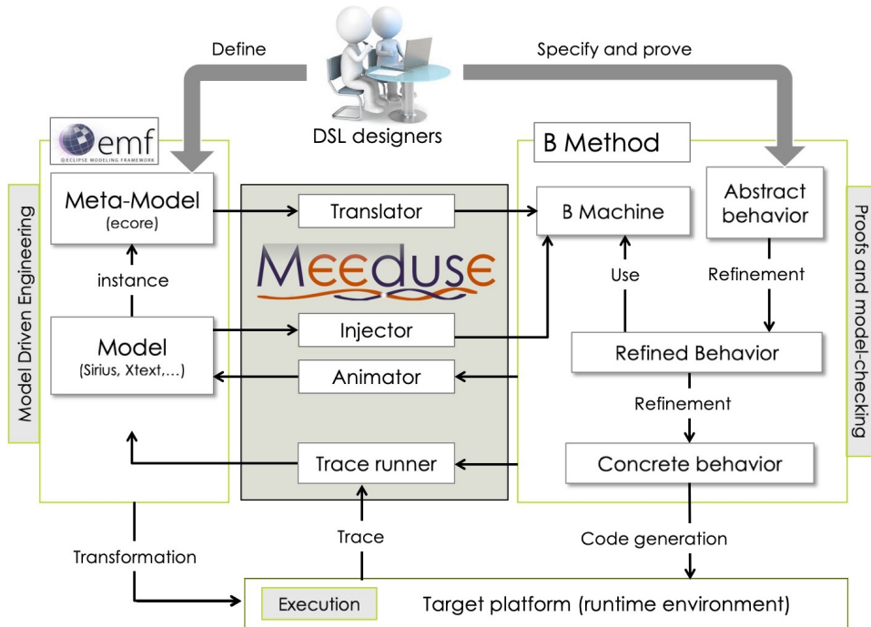
Figure 4.1: Meeduse overview
