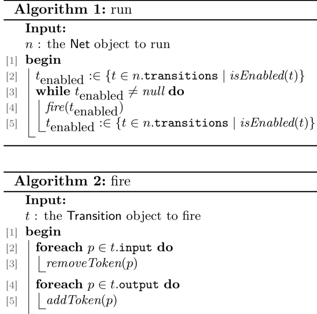
Figure 4.4: Running a Petri-net.
