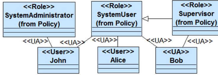
Figure 3.3: Users assignement
