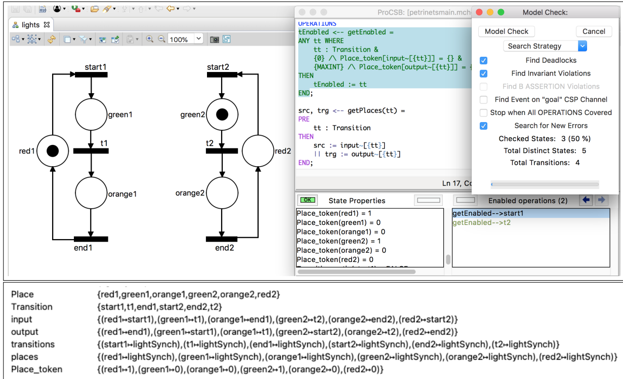
Figure 4.13: Integration of ProB within EMF
