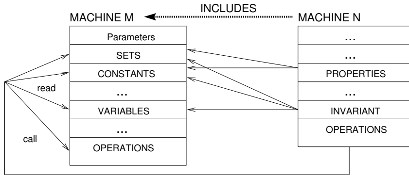
Figure 1.2: Clause INCLUDES.
