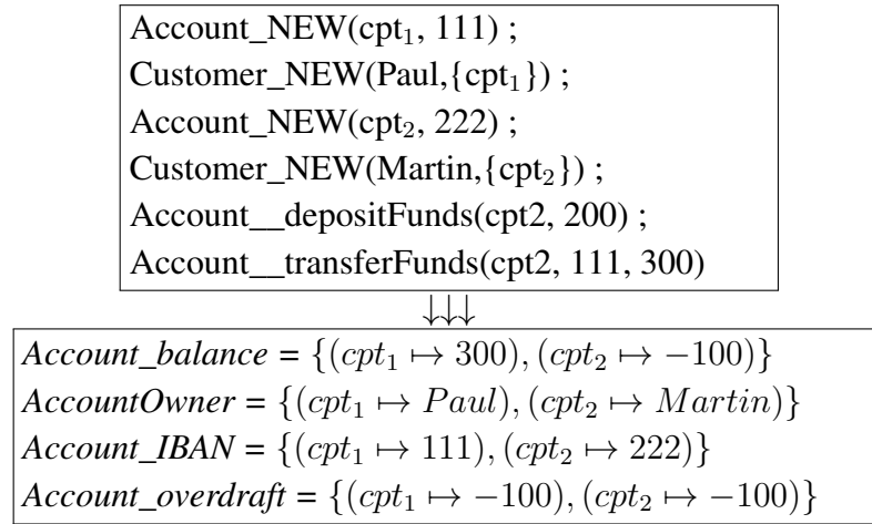
Figure 2.18: Valid functional sequence and its target state
