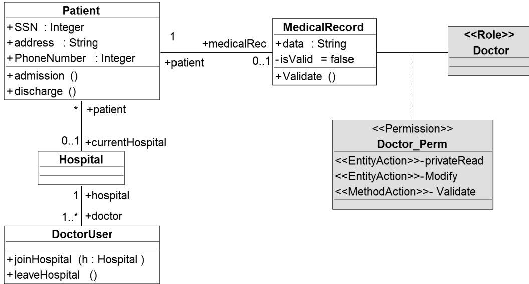
Figure 2.2: Functional model enriched by RBAC rules
