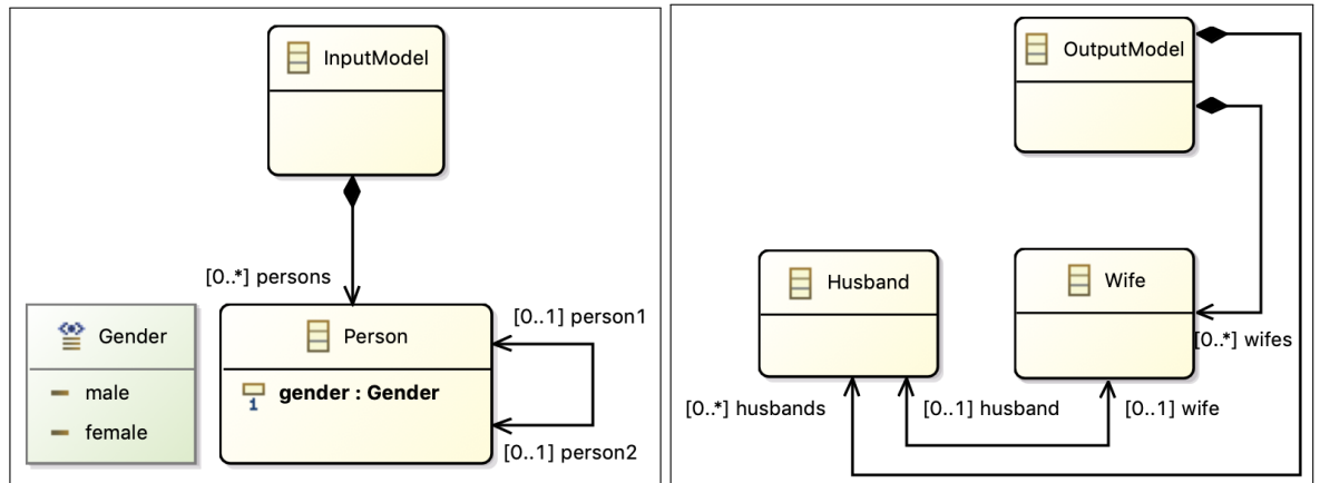
Figure 5.15: Input/Output meta-models
