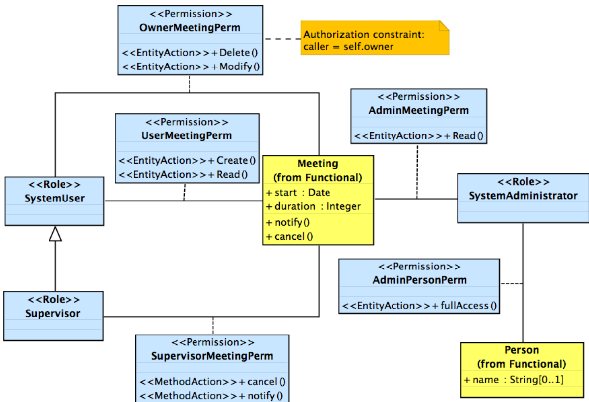
Figure 3.2: Security model of meeting scheduler system
