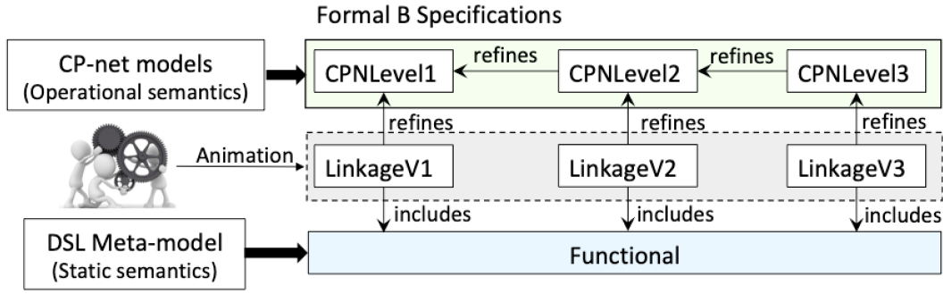
Figure 5.9: Merging CP-Nets and DSLs in a formally defined framework
