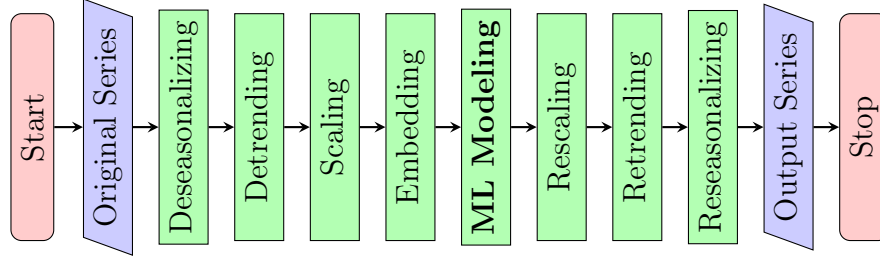
Figure 5.1: Flowchart of the machine learning pipeline.
