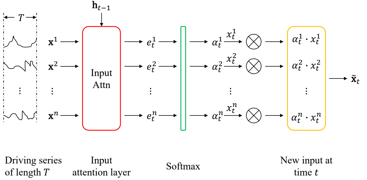
Figure 6.1: DA-RNN's Input Attention Mechanism.
