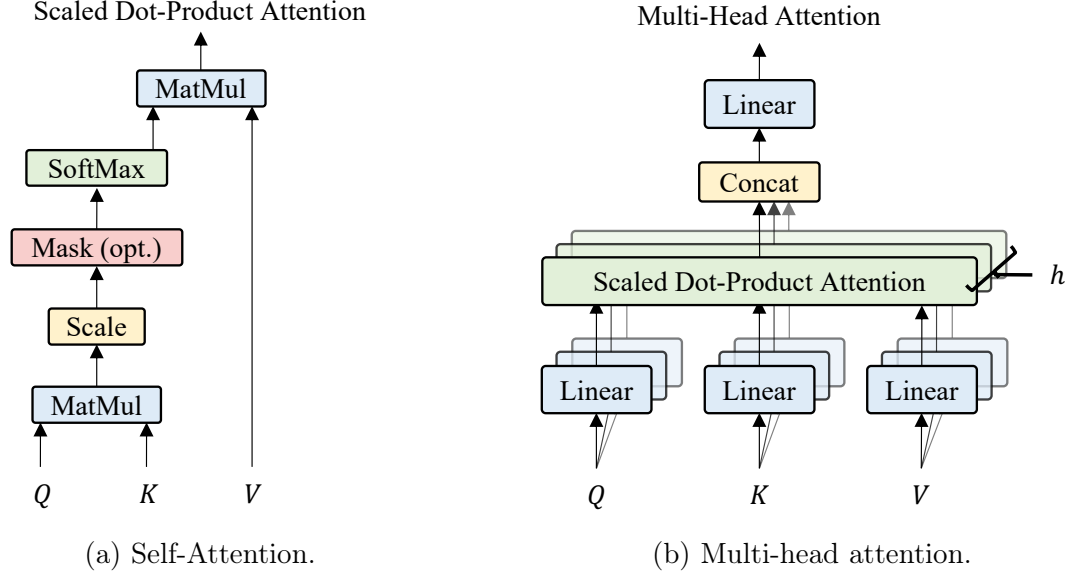
Figure 4.7: Attention mechanism in Transformer.
