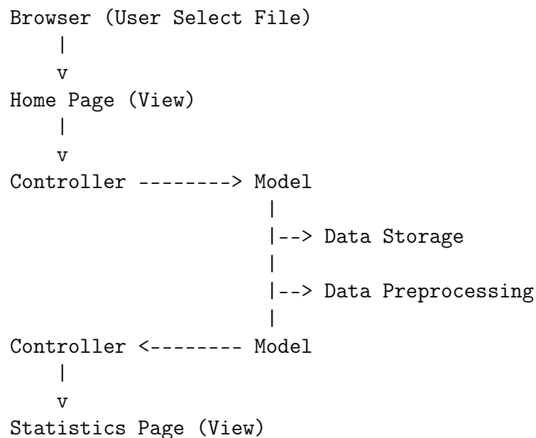
Figure 8.6: The data uploading process.
