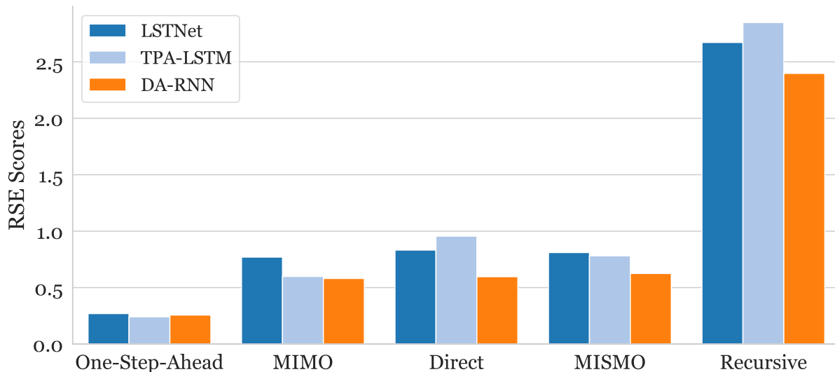
Figure 6.5: Average RSEs over the horizon for different strategies.
