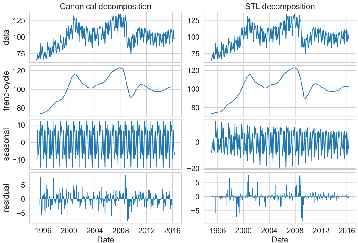
Figure 3.12: Comparison of canonical and STL decomposition of the production of electrical equipment in the EU.
