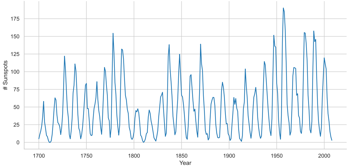
Figure 3.1: Sunspots data from the National Geographic Data Center.
