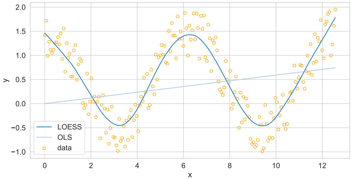
Figure 3.10: A LOESS example.
