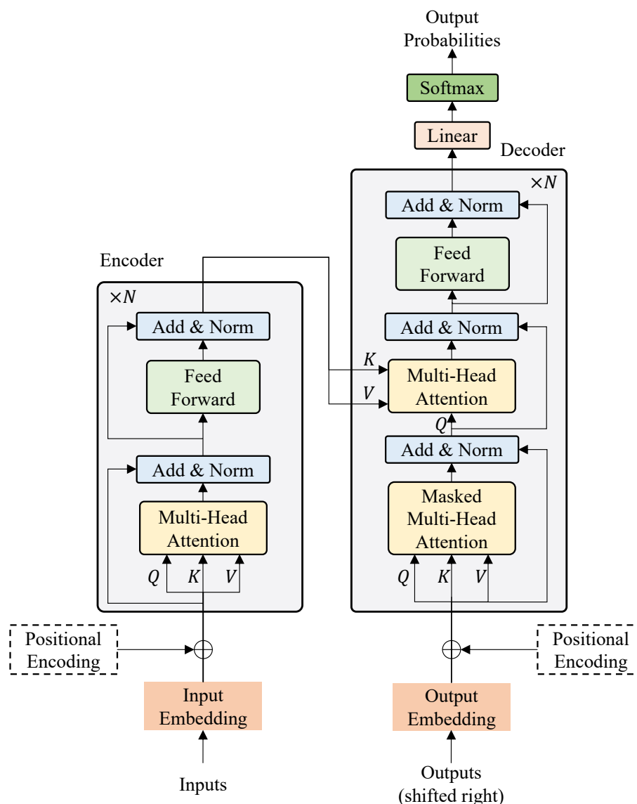
Figure 4.6: The architecture of Transformer.
