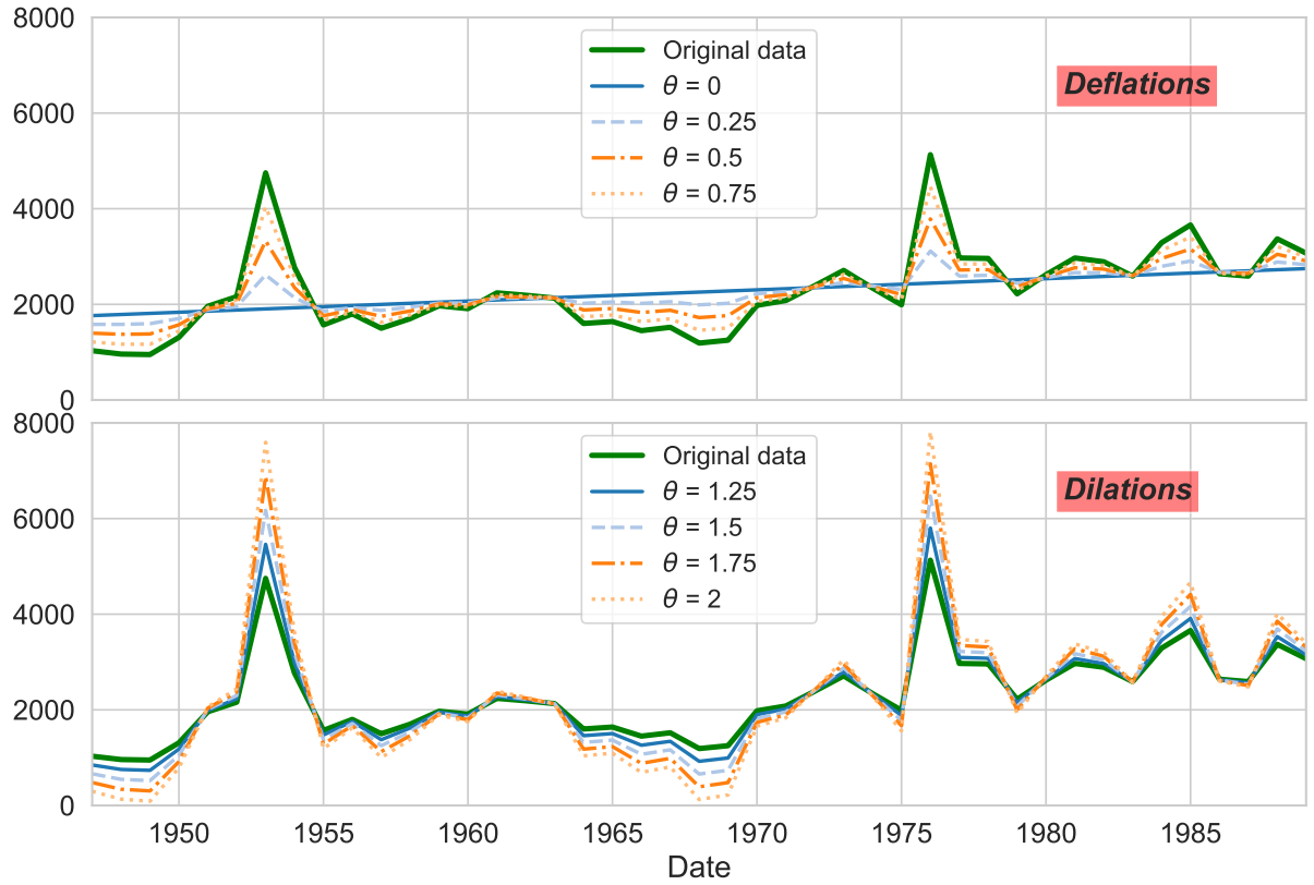
Figure 3.13: Theta lines deflations and dilations of the Series N200 in M3-Competition.
