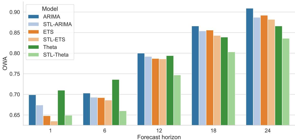
Figure 5.3: OWAs for STL decomposition on econometric models.
