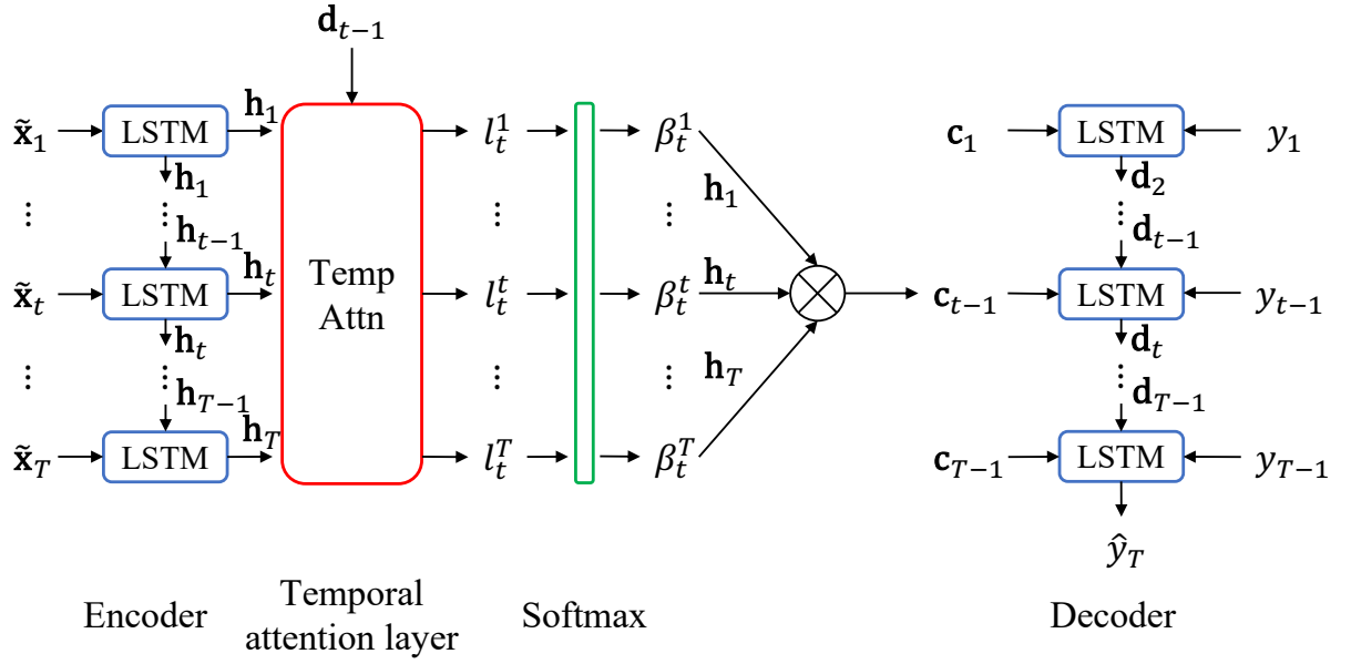
Figure 6.2: DA-RNN's Temporal Attention Mechanism.
