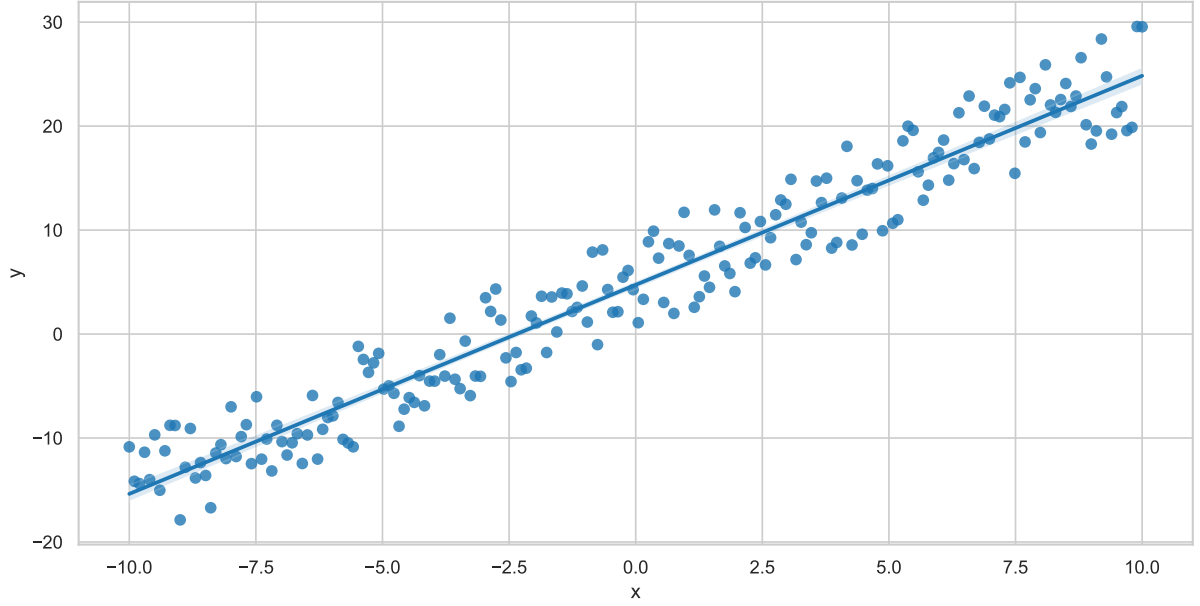
Figure 3.3: An example of linear regression on a synthetic dataset.
