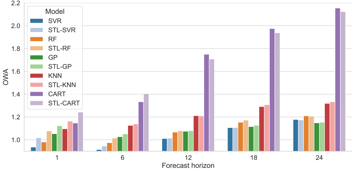
Figure 5.4: OWAs for STL decomposition on machine learning models.
