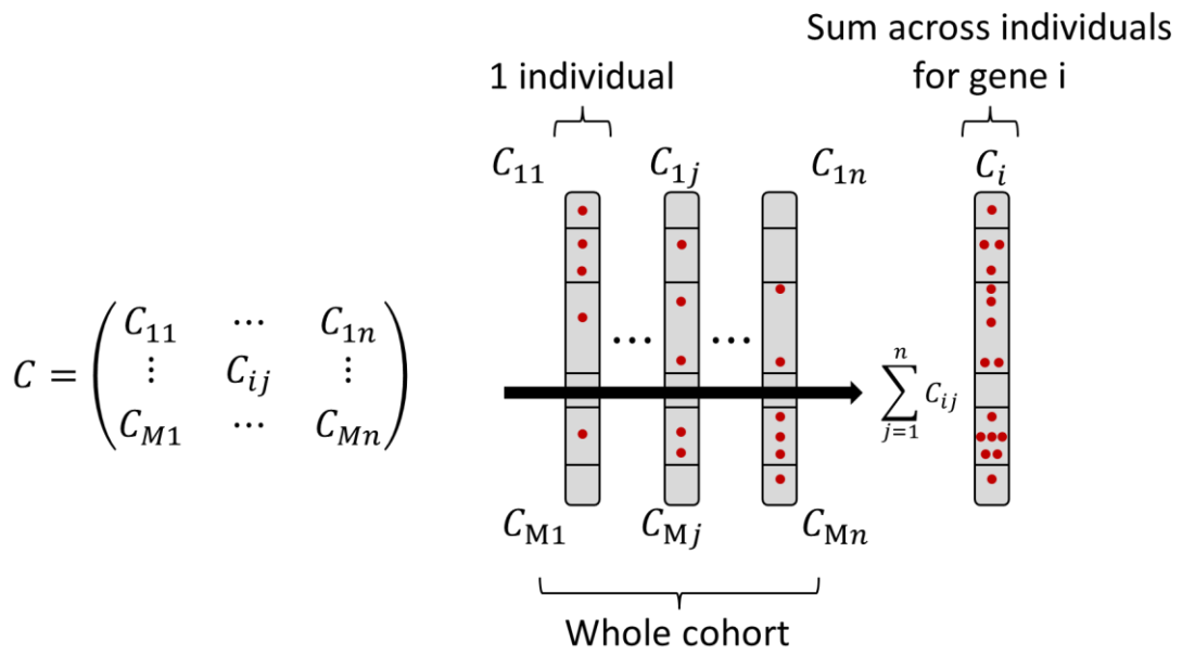
Figure 10: Conceptual diagram of the intuition behind the case-only burden test
