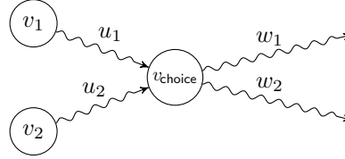
◆ Figure 29. A game \mathcal{G} in which Eve cannot play optimally using positional strategies if \text{Res}(W) is not totally ordered. ◀
