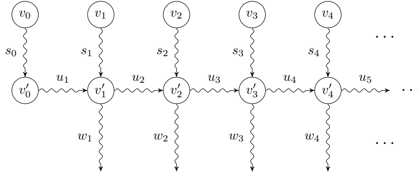
◆ Figure 45. Game in which Eve wins if she produces a non-strictly increasing sequence of numbers. She can win from every v_i , but not positionally.
