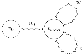
◆ Figure 40. A game \mathcal{G} in which Eve cannot play optimally using positional strategies if \mathcal{A} is not fully progress consistent.
