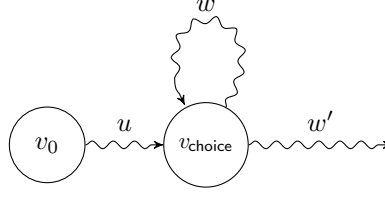
◆ Figure 31. A game \mathcal{G} in which Eve cannot play optimally using positional strategies if W is not progress consistent.
