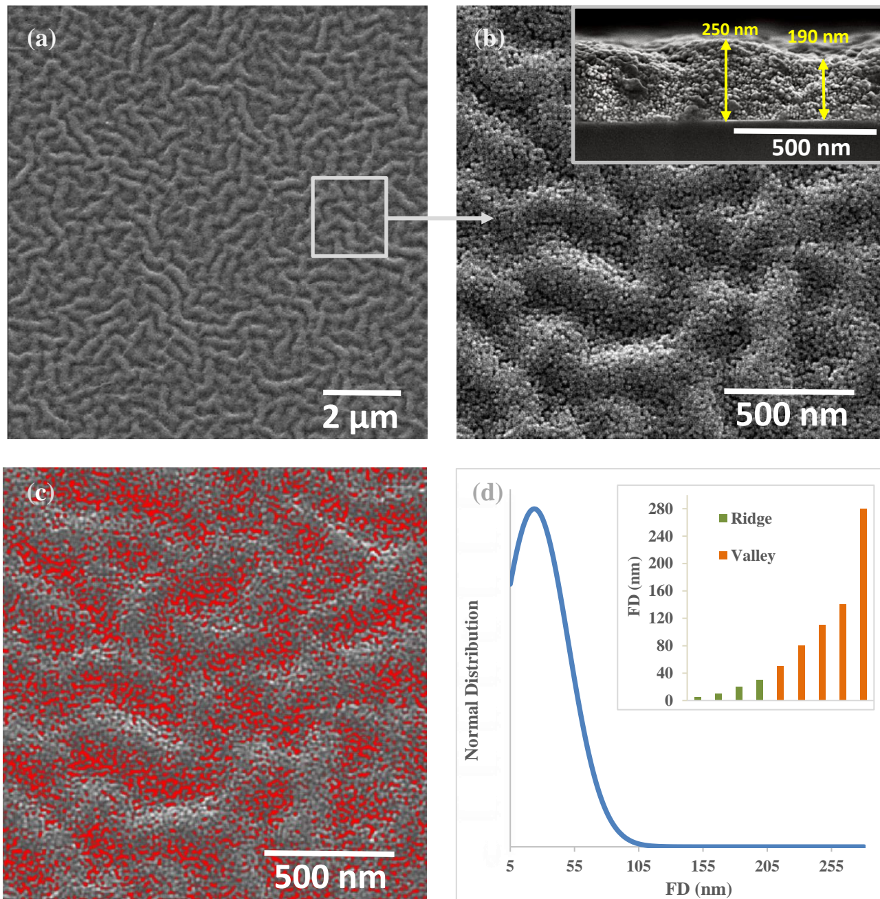
Figure 1. (a) SEM top view image for 7 layers' ZnO thin films after post-heat treatment at 450 °C, (b) Zoomed-in view of "a", the inset represents a cross-sectional view of figure 1b, (c) Pores distribution on ridges and valleys by treating Figure 1b using Image J software, (d) Pores' Feret diameter (FD) distribution from figure 1, the inset represents the FD of distributed pores between ridges and valleys.
