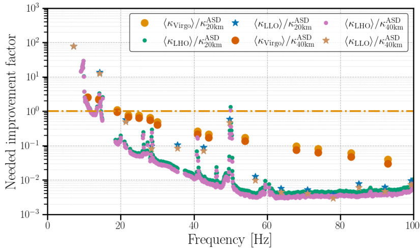
Fig. 8.5.: Needed improvement factor as a function of frequency for the 'ASD' upper limits on the CE magnetic coupling function. The dash-dotted orange line indicates the line where no improvement is necessary. We have used the 40km and 20km design sensitivities as presented in [335] and which are accessible in [233].
