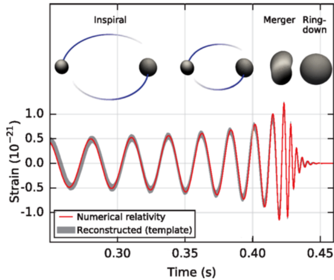
Fig. 3.1.: Estimated gravitational-wave strain amplitude from GW150914 projected onto the LIGO Hanford detector. The inset images show numerical relativity models of the black hole horizons as the black holes coalesce. Figure and caption taken and modified from [19], under the terms of the Creative Commons Attribution 3.0 License.
