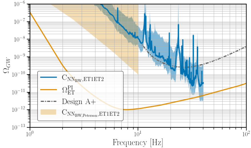
Fig. 9.16.: The projected impact from correlated NN from body-waves. The blue line represents the median value and the associated surface is delimited by the 10% and 90 % percentiles. As a comparison we also make the same projection using the Peterson low noise and high noise models. For the broadband ( \Omega_{ET}^{PI} ) sensitivity to a GWB we assumed one year of observation time (100% duty cycle). The one year PI curve of the A+ design for the LIGO Hanford, LIGO Livingston and Virgo detectors is represented by the dot-dashed curve. This curve was obtained using the open data provided by the LVK collaborations [243] and was first presented in [30]. Please note: in this chapter we present the 1\sigma PI-curve, whereas in [30] and in Fig. 8.6 the 2\sigma PI-curve is shown.
