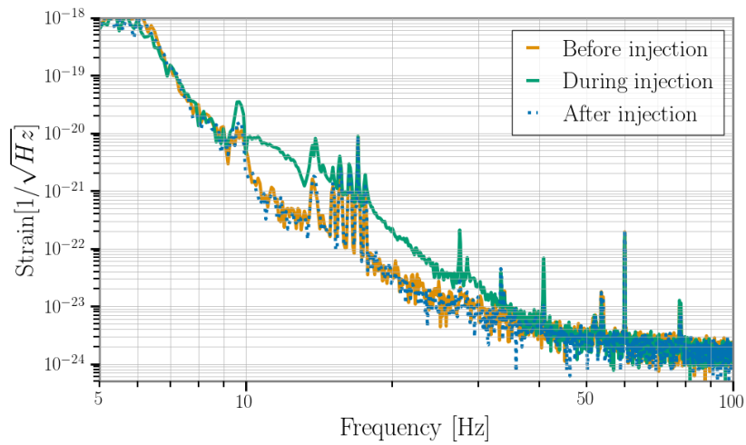
Fig. 7.10.: \text{CSD}^{1/2} between the observed strain at LHO and LLO. The CSD is calculated during a five minute window before (orange), during (green) and after (blue, dotted) the magnetic injection.
