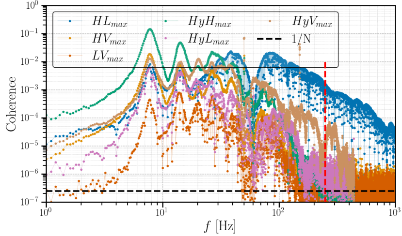
Fig. 7.1.: Coherence spectrum between HL (blue), HV (orange), LV (red), Hylaty-LHO (green), Hylaty-LLO (purple) and Hylaty-Virgo (brown). At each frequency the maximal coherence of the four magnetometer pairs is plotted for a given baseline. In the absence of correlated noise, one expects this to be consistent with Gaussian noise given by the inverse of the number of averages ( N ) used to make the coherence spectrum, indicated by the black dashed line. Data spans April 2 2019 00:00:00 UTC to March 27 2020 00:00:00 UTC, consistent with the overlap between LIGO's and Virgo's third observing run (also including data from the commissioning break during October 2019). Above 250Hz, the magnetometers at the Hylaty experience significant loss in sensitivity.
