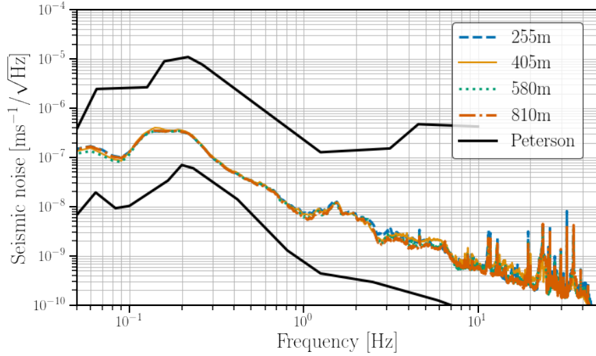
Fig. 9.11.: The median \text{CSD}^{1/2} of the underground (depth \approx 610\text{m} ) seismometers as a function of the horizontal distance. The data (March 2015 to Dec 2016) are analysed using 100 second long segments which are averaged per 24h-window. As a comparison, the Peterson low and high noise models [210] are shown in black.
