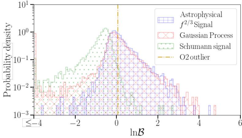
Fig. 10.6.: Probability density of \ln \mathcal{B} for an astrophysical \alpha = 2/3 power-law signal, random draws from a Gaussian process using our optimized (most conservative) SE-kernel and a Schumann signal. The lowest bin contains all \ln \mathcal{B} \leq -4 . For each signal type 5000 injections were performed with an injection strength of \text{SNR}=1.25 . The choice of \alpha = 2/3 and \text{SNR}=1.25 matches the parameters of observed outlier of the O2 results for an isotropic GWB [14]. For a low SNR outlier the GW Geodesy tool has very limited power, as can be seen by the high level of overlap between the Gaussian process and the astrophysical signal distributions. However, it can be confidently excluded that the O2-outlier was caused by a Schumann signal.
