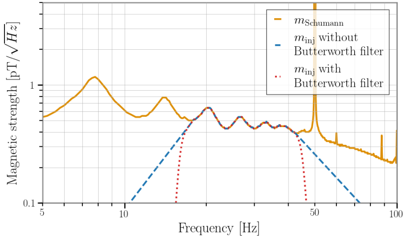
Fig. 7.11.: The magnetic spectrum, m_{\text{inj}} , that will be used to inject coherently between multiple GW detectors to test how correlated noise affects GWB pipelines. The spectrum is compared to the Schumann resonance spectrum observed at Sos Enattos (10% scaled to 95% amplitude, see Fig. 7.3). Furthermore m_{\text{inj}} is shown both before as well as after applying the 32nd order low- and high-pass Butterworth filters.
