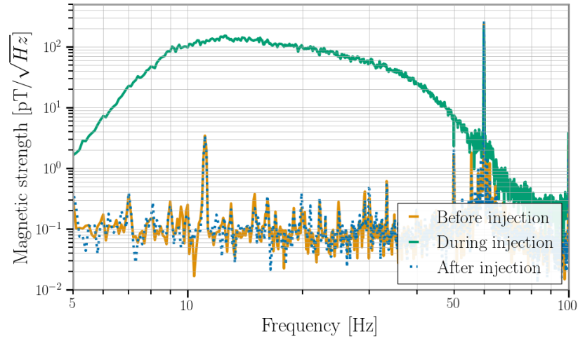
Fig. 7.8.: CSD^{1/2} between a magnetometers at LHO and LLO. At both sites a single magnetometer was used, pointing along the x-arm of the respective detector. More specifically the used sensors are: H1:PEM-CS_MAG_IVEA_VERTEX_X_DQ and L1:PEM-CS_MAG_IVEA_VERTEX_X_DQ. The CSD is calculated during a five minute window before (orange), during (green) and after (blue, dotted) the magnetic injection.
