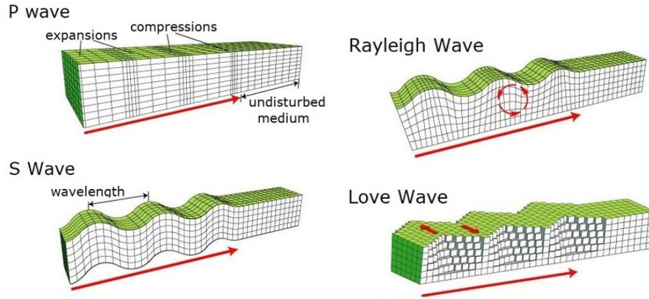
Fig. 5.3.: Illustration of P-, S_V -, Rayleigh- and Love-waves. Figure taken from [353]. ©Science Learning Hub – Pokapū Akoranga Pūtaiao, University of Waikato.
