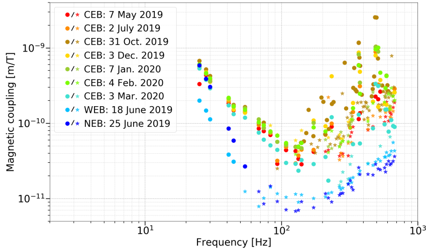
Fig. 7.4.: Magnetic coupling functions for CEB, WEB and NEB. For CEB multiple injections over the time of O3 are shown to illustrate the time variations. Dots are measured values of the magnetic coupling, while stars are upper-limits, calculated using Eq. 7.2.
