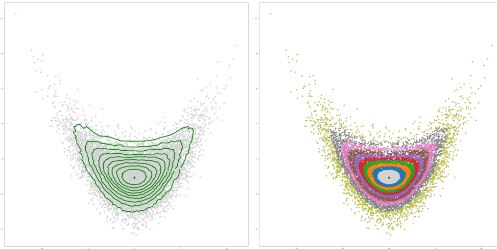
Figure 7.1.1: Quantile contours \mathcal{C}_{\pm}(\tau) (left panel) and regions \mathbb{C}_{\pm}(\tau) (right panel) for the banana-shaped Gaussian mixture of Section 7.4.1.2 and the quantile orders \tau = 0.1, 0.2, \dots, 0.9 .
