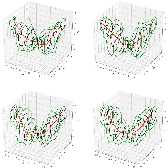
Figure 7.4.3: Estimated quantile contours (Model (7.21)) based on k -nearest neighbors weight functions for different choices of k . The sample size is n = 3601 ; k = 101 (upper left panel), k = 256 (upper right panel), k = 401 (lower left panel) and k = 625 (lower left panel). The estimated contour orders are \tau = 0.2 (black) and 0.4 (green); the estimated conditional center-outward medians are shown in red.
