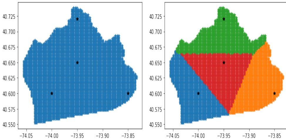
Figure 3.4.1: In the left original data of the sample m = 3 , 129 of Brooklyn's population distribution. On the Right, the empirical Laguerre cells \text{Lag}_i^R(\mathbf{z}^*) for the fountains located at (-74.0, 40.6) (blue), at (-73.85, 40.6) (orange), at (-73.95, 40.72) (green) and at (-73.95, 40.65) (red). Black points represent the fountains.
