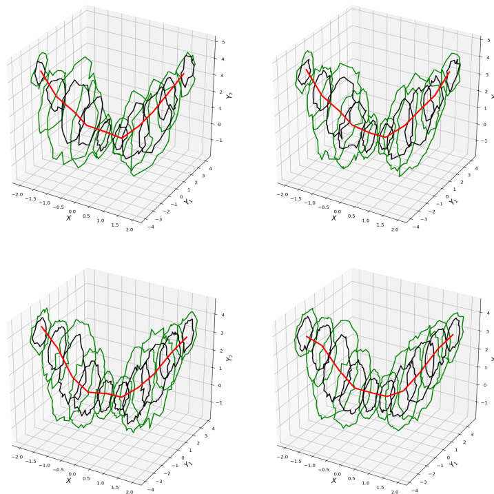
Figure 7.4.2: Estimated quantile contours (Model (7.21)) based on Gaussian kernel weight functions for different choices of the bandwidth h . The sample size is n = 3,601 ; bandwidth values are h = 0.05 (upper left panel), h = 0.1 (upper right panel), h = 0.2 (lower left panel) and h = 0.3 (lower right panel). The estimated contour orders are \tau = 0.2 (black) and 0.4 (green); the estimated conditional center-outward medians are shown in red.
