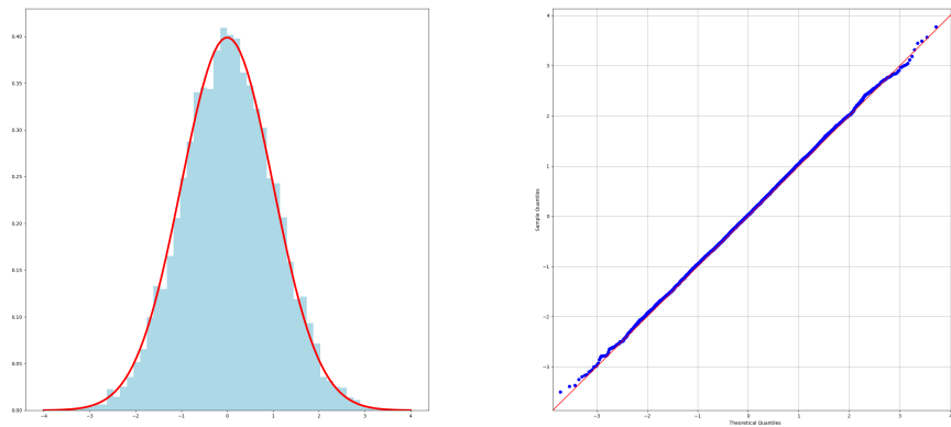
Figure 3.5: Illustration of Theorem 3.2.2 using bootstrap procedures. Histograms (left) and Q–Q plot (right) of the bootstrap estimation of \sqrt{m} \frac{W_2^2(P, Q_m) - W_2^2(P, Q)}{\sigma_2(Q_m; \mathbf{z}^m)} .
