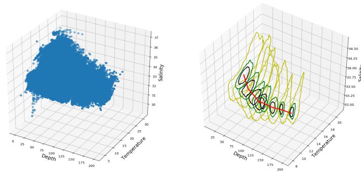
Figure 7.4.8: CalCOFI dataset. Left panel: the original dataset ('depth,' 'temperature,' 'salinity') for 'depth' \leq 200 (sample size for 'depth' \leq 200 , dropping empty values, is n = 505,829 ). Right panel: the empirical conditional center-outward quantile contours of orders \tau = 0.2 (black), \tau = 0.4 (green), and \tau = 0.8 (yellow) and the empirical conditional center-outward median (red) for the multiple-output regression of (Y_1, Y_2) = ('temperature,' 'salinity') with respect to X = 'depth.' Estimation based on a k -nearest neighbors weight function with k = 6,401 .
