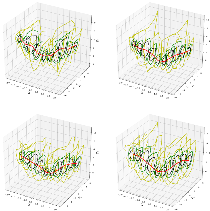
Figure 7.4.6: Performance, in Model (7.23), of the k -nearest neighbors weight functions-based estimation for various choices of k . The sample size is n = 3601 ; k = 101 (upper left panel), k = 256 (upper right panel), k = 401 (lower left panel), and k = 625 (lower left panel). The empirical contour levels are \tau = 0.2 (black), 0.4 (green), and 0.8 (yellow); the estimated conditional center-outward medians are shown in red.
