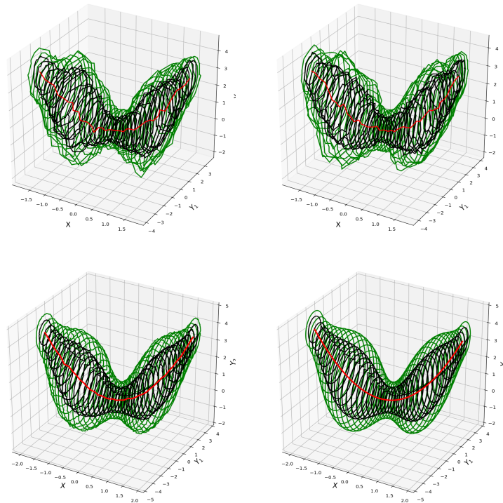
Figure 7.4.1: Estimated (sample sizes 3,601 in the upper left panel, 10,000 in the upper right panel, 128,020 in the lower left panel) and population (lower right panel) quantile contours of order \tau = 0.2 (black) and 0.4 (green) for Model (7.21); the (estimated) conditional center-outward medians are shown in red. Estimations are based on the k -nearest neighbors weights (ii) with N = k = 401, 1,000, and 6,401 and n = 3,601, 10,000, and 128,020, respectively.
