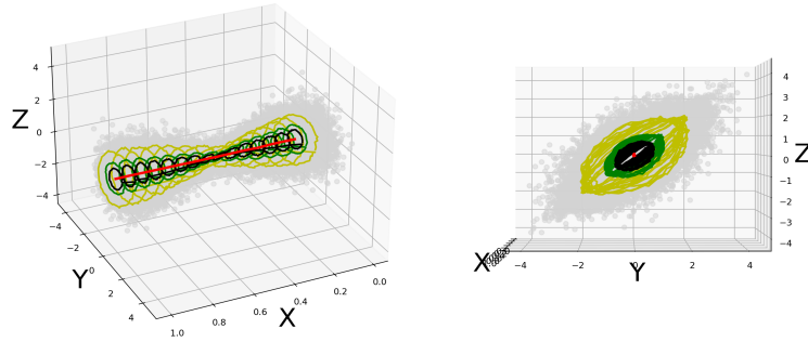
Figure 1.3: Example of univariate quantile regression; with X and \mathbf{Y} = (Y, Z) as in (1.26). The number of observed points is n = 7,000 . The quantile contours for \tau = 0.2, 0.4, 0.8 are represented in black ( \tau = 0.2 ), green ( \tau = 0.4 ) and yellow ( \tau = 0.8 ). The center is represented in red.
