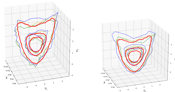
Figure 7.4.7: Comparison between the empirical conditional contours \hat{C}_{\pm}^{(n)}(\tau | 0) (levels \tau = 0.2, 0.4, 0.8 ; sample size n = 3,601 ) in Model (7.23) based on Gaussian kernel weight functions (bandwidths h = 0.1 (green), h = 0.2 (yellow), and h = 0.3 (blue)) (left panel) and those in Figure 7.4.4, based on k -nearest neighbors weight functions ( k = 226 (green), k = 485 (yellow), and k = 901 (blue)); sample size n = 576,040 ) (right panel). The center-outward quantiles of Figure 7.4.4 (to be considered as population values) are shown in red.
