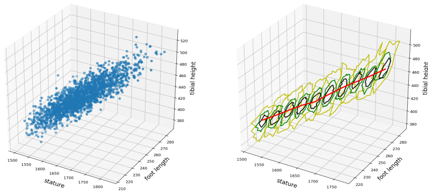
Figure 7.4.10: ANSUR 2 dataset (sample size n = 1,986 ). Left panel: the original dataset of X = \text{'stature'} and (Y_1, Y_2) = (\text{'foot length,' 'tibial height'}) . Right panel: the empirical conditional center-outward quantile contours of orders \tau = 0.2 (black), \tau = 0.4 (green), \tau = 0.7 (yellow) and the empirical conditional center-outward median (red) for the multiple-output regression of (Y_1, Y_2) with respect to X ; estimation based on a Gaussian kernel weight function with bandwidth h = 15 .
