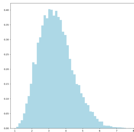
Figure 3.6: Illustration of Theorem 3.1.4, by using Monte Carlo's method, for Q with disconnected support.
