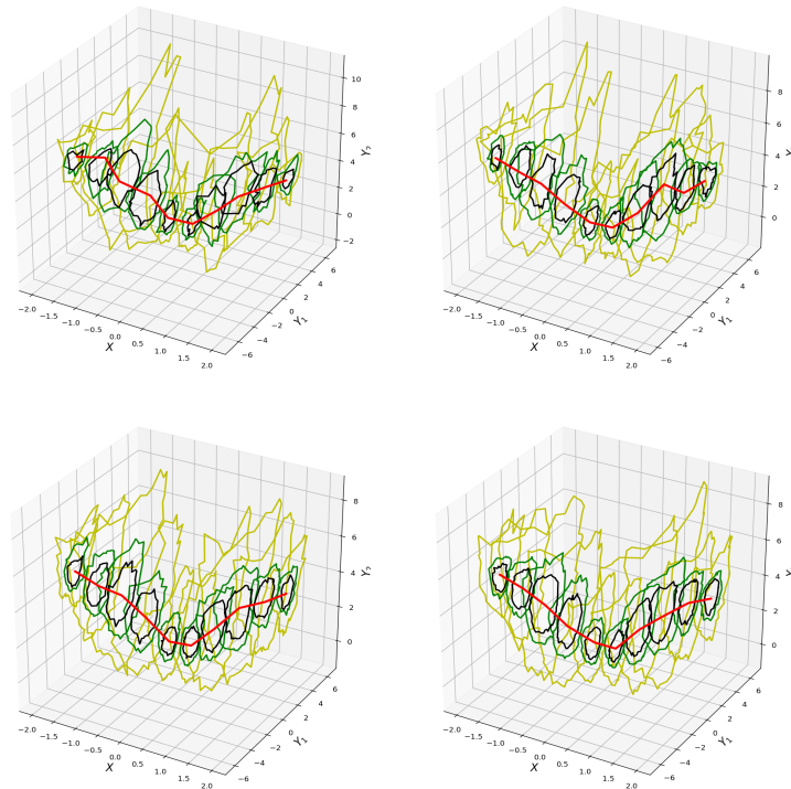
Figure 7.4.5: Performance, in Model (7.23), of Gaussian kernel weight functions-based estimation for various choices of the bandwidth. The sample size is n = 3,601 , and the bandwidths are h = 0.05 (upper left panel), h = 0.1 (upper right panel), h = 0.2 (lower left panel), and h = 0.3 (lower right panel). The empirical contour levels are \tau = 0.2 (black), 0.4 (green) and 0.8 (yellow); the estimated conditional center-outward medians are shown in red.
