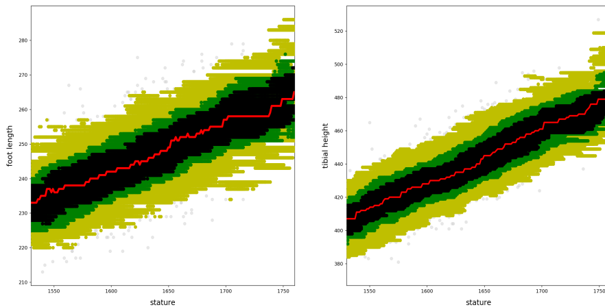
Figure 7.4.11: ANSUR 2 dataset (sample size n = 1,986 ). Left panel: projection of the empirical center-outward quantile regions (orders \tau = 0.2, 0.4, 0.8 ) and median on the axes ( \text{'stature,' 'foot length'} ), for the multiple-output regression of (Y_1, Y_2) = (\text{'foot length,' 'tibial height'}) with respect to X = \text{'stature'} . Right panel: projection of the same on the axes ( \text{'stature,' 'tibial height'} ); see Figure 7.4.10 for the color code.
