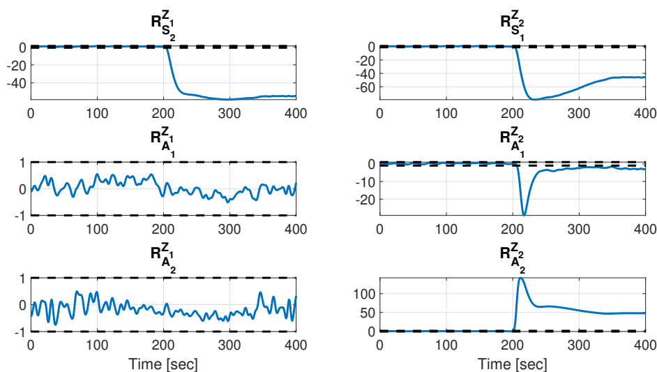
FIGURE 4.17: Case B: multiplicative fault on sensor S_2 at time t = 200s with normalized thresholds
