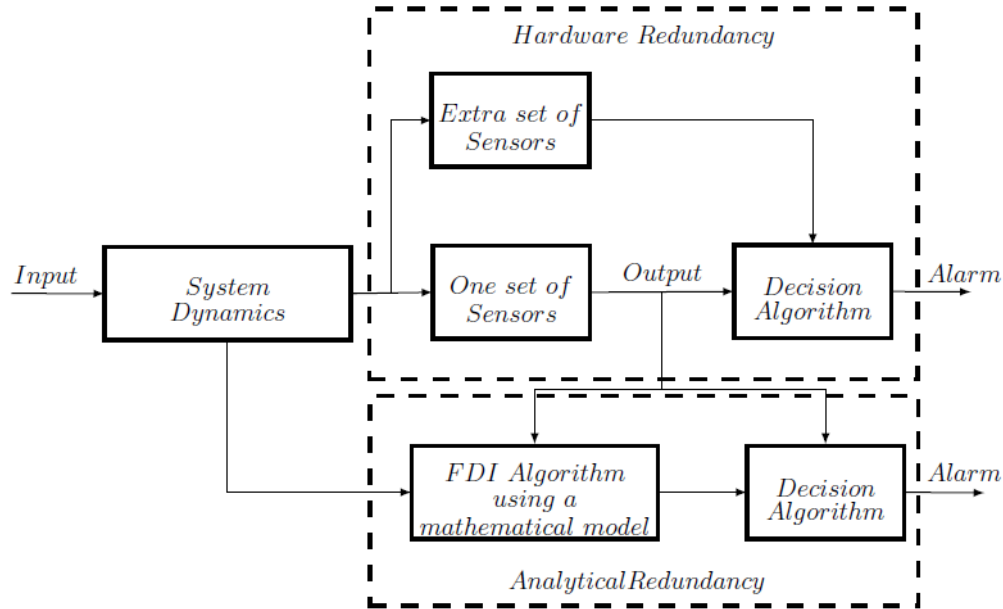
FIGURE 1.2: Hardware redundancy and analytical redundancy diagram (Torres, 2014)
