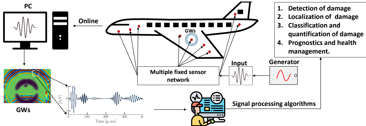
Figure 1.3: Schematic of active GWs based SHM.
