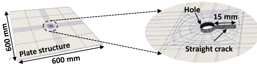
Figure 4.8: Crack length of 15 mm from hole mesh configuration obtained from CIVA.
