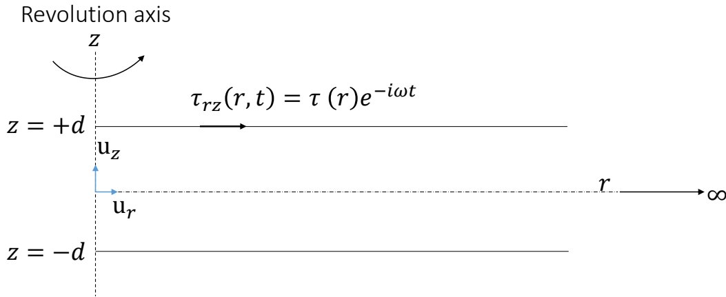
Figure 2.1: Axisymmetric structure.
