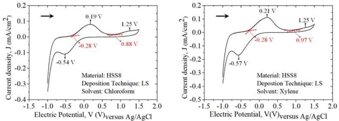
Figure 43. Cyclic voltammogram for LS films of HSS8 (30 layers) solubilized in chloroform (to the left) and xylene (to the right).
