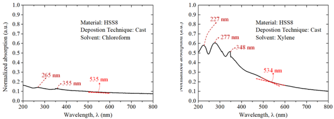
Figure 46. Absorption spectra for cast films of HSS8 solubilized in chloroform (to the left) and xylene (to the right).
