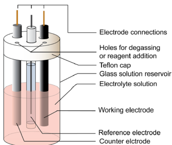
Figure 19. An electrochemical cell setup for CV experiments.
