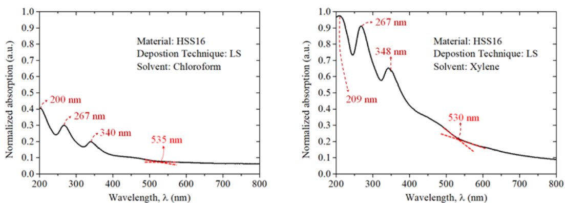
Figure 49. Absorption spectra for LS films of HSS16 solubilized in chloroform (to the left) and xylene (to the right).
