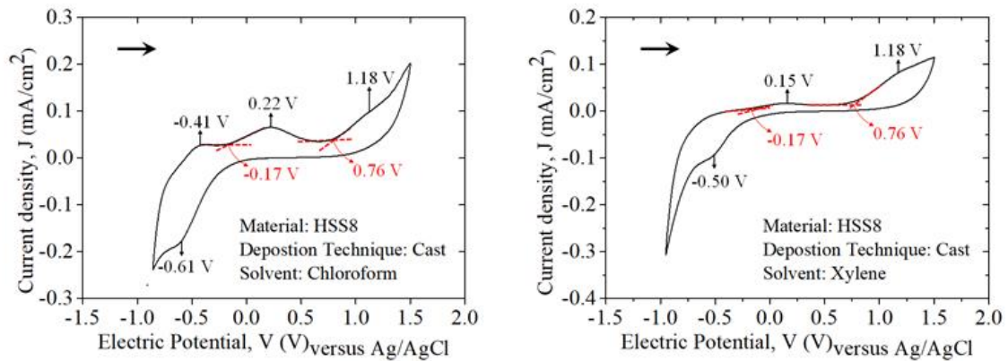
Figure 42. Cyclic voltammogram for cast films of HSS8 solubilized in chloroform (to the left) and xylene (to the right).
