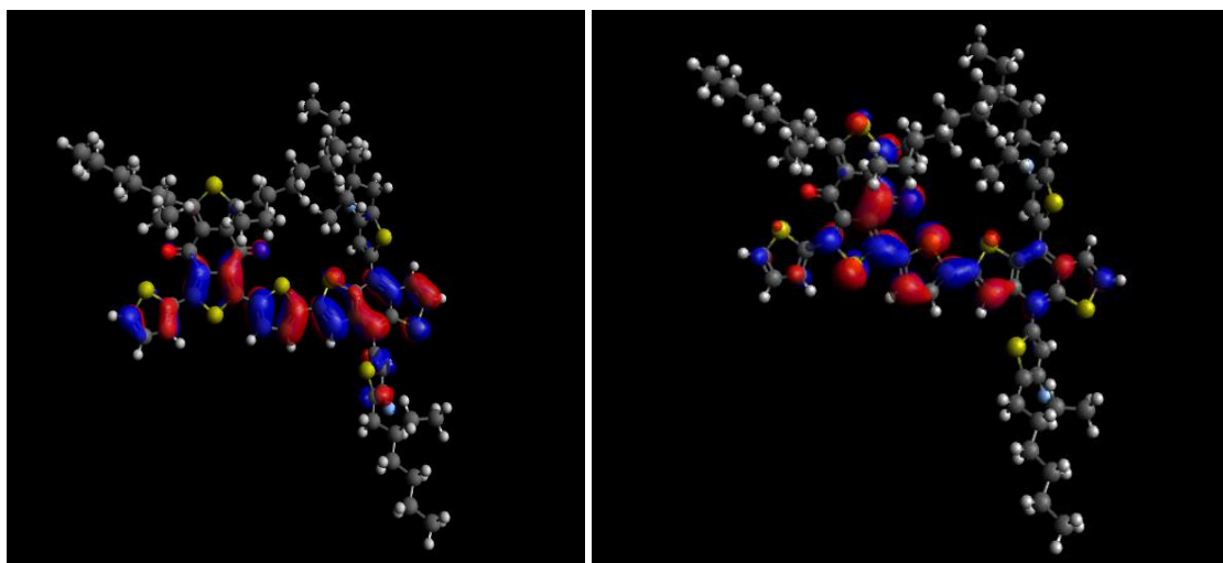
Figure 23. HOMO (to the left) and LUMO (to the right) orbitals of PM6 monomer.
