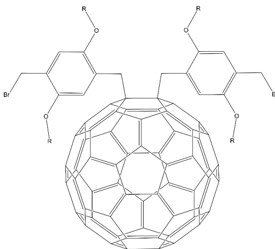
Figure 13. Molecular structure of di-bromo monomer.
