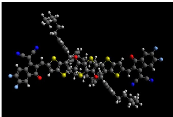
Figure 30. Optimized structure of O6T-4F monomer.
