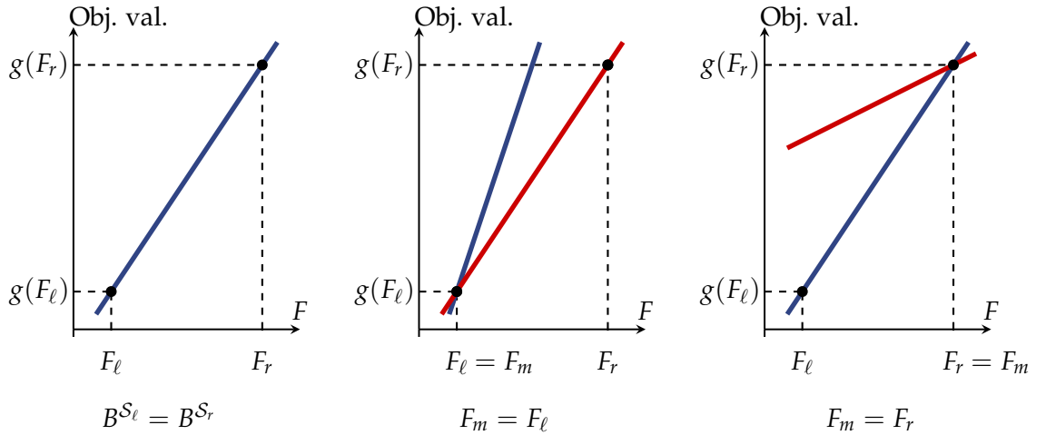
Figure 3.3: Illustration of the situations that can occur when EX-PLORE( F_\ell, \mathcal{S}_\ell, F_r, \mathcal{S}_r ) is run
