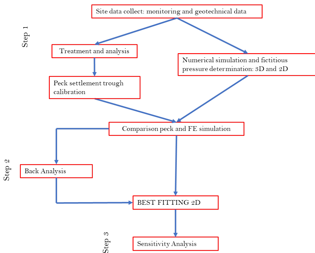
Figure 3.1: TBM induced settlement analysis chart
