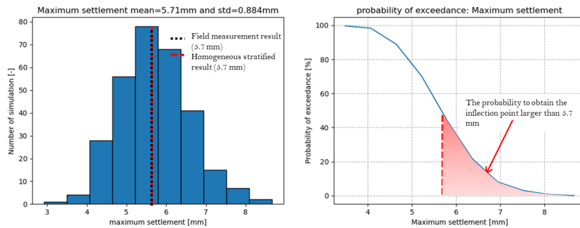
Figure 3.33: Histogram of the maximum settlement and cumulative distribution function
