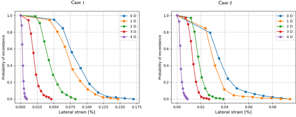
Figure 5.18: Probability of exceedance at various levels of the lateral strain; Case 1: spatial variable models calculated with a lower confinement pressure, and case 2: spatial variable models calculated with a higher confinement pressure
