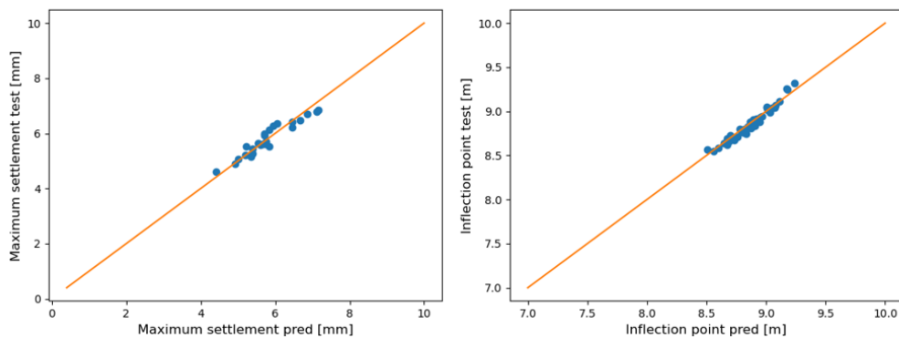
Figure 4.10: Meta model predictions vs FE results for the stratified homogeneous layers with 25 clusters
