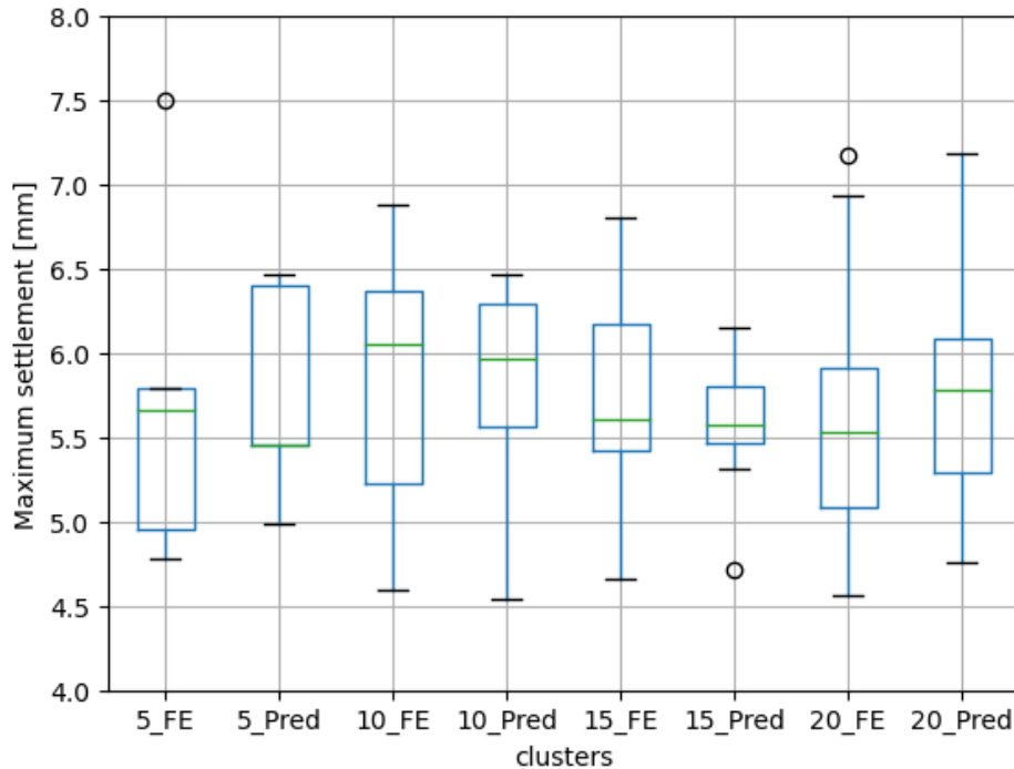
Figure 4.12: Maximum settlement box plot of the FE results (FE) and the predictions (Pred) for the spatial variability model according to a selected number of clusters
