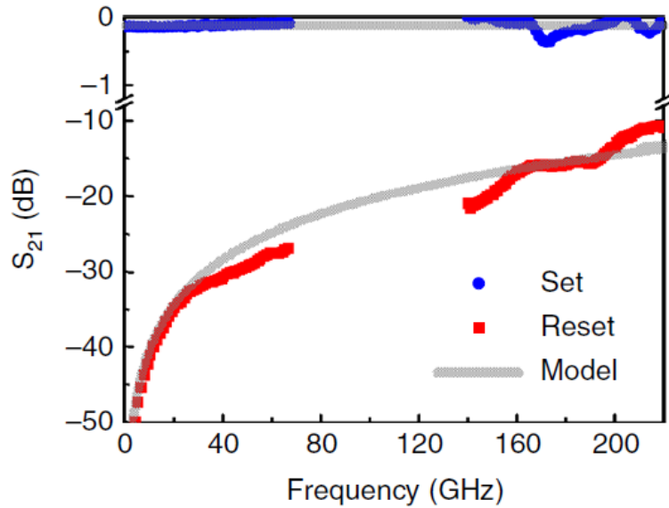
Figure 9 Measured S-parameter data and simulated result from 0-67 GHz and 140-220 GHz from [3]
