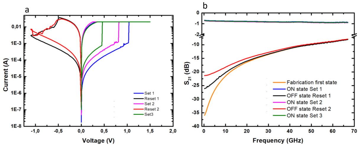
Figure 5 (a) I-V characteristics with multiple cycle on the same 1 \times 1 \mu\text{m}^2 device for the Au/MoS 2 /Pt interface. (b) S_{21} parameters of Au/MoS 2 /Pt interfaces with multiple cycle on the same device. Device size of 1 \times 1 \mu\text{m}^2 active part. The insertion loss of this device is -0.9 dB at 67 GHz and the isolation is -8dB at 67 GHz.
