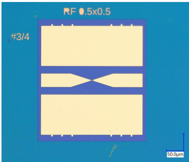
Figure 11 Optical microscopy image of a 0.5 \times 0.5\text{ }\mu\text{m}^2 RF switch with coplanar waves guides taken from batch SS03.
