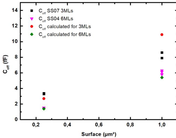
Figure 29 Comparison of C_{OFF} for SS07 (3 MLs) and SS04 (6 MLs) for the fabrication state with the interface Ni/MoS 2 /Pt. The calculation and the extracted value are close to each other with a value of 3fF for the calculated and the measured C_{OFF} for a 0.25x0.25 μm 2 device for example.
