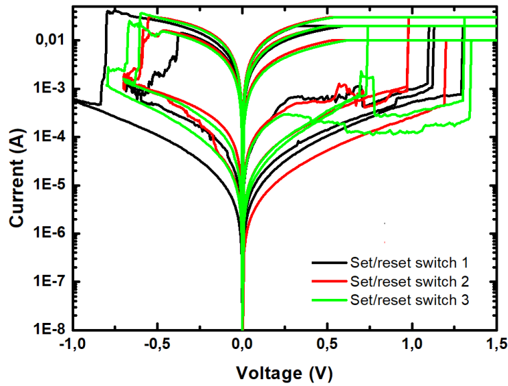
Figure 20 Summary of I-V characteristics of three different 0.5 \times 0.5 \mu\text{m}^2 devices with Au/MoS 2 /CrAu interface. Multiple switching cycles of these three devices are displayed. The switching voltage from its OFF to ON state is between 0.5 V and 1.5 V. The switching voltage from its ON state to OFF state is between -1 V and -0.5 V.
