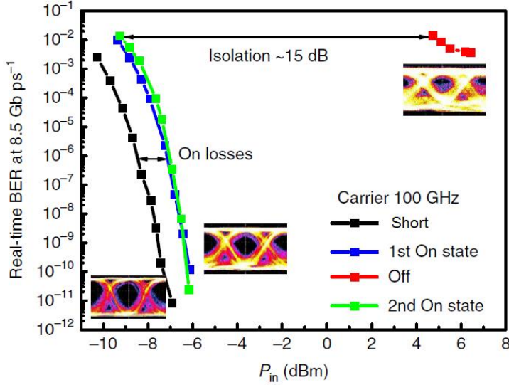
Figure 13 BER measurement with different switch status inset: eye diagram measured at f_c = 100 GHz with a data rate of 8.5 Gbit.s -1 from [3]
