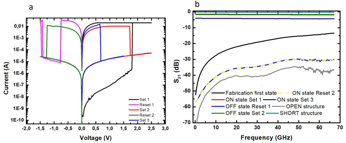
Figure 21 (a) I-V characteristics with multiple switching for one 1 \times 1 \mu\text{m}^2 device with Ni/MoS 2 /Pt interface. (b) S_{21} of Ni/MoS 2 /Pt interfaces for one 1 \times 1 \mu\text{m}^2 device and compared to the SHORT/OPEN structure fabricated on chip. Multiple switching cycle of a devices are displayed. The insertion loss value is -1.6 dB at 67 GHz and the isolation is -30 dB at 67 GHz for RESET 1.
