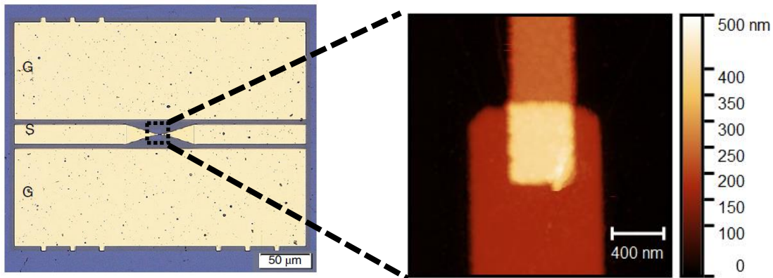
Figure 8 Optical microscopy image of an \text{MoS}_2 RF switch with GSG Au electrode from [6] (b) Representative AFM image of the active part region with 0.5 \times 0.5 \mu\text{m}^2 active part area
