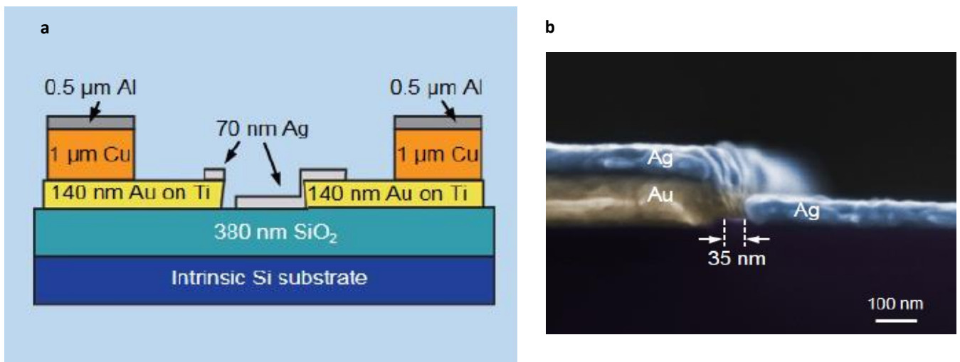
Figure 14 (a) cross view of a gap CBRAM switch. (b) Colored view of a SEM image of a CB switch from [28]
