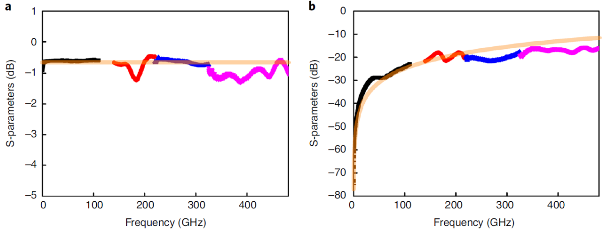
Figure 10 S-parameters of a MoS 2 nonvolatile switch. De-embedded S_{21} data in (a) ON state and (b) OFF state. The SET and RESET data are measured on a device with a 0.2 \times 0.2 \mu\text{m}^2 active part area. Black, red, blue and magenta colour lines show S_{21} data from the 0.25-110, 140-220-220-325 and 325-480 GHz bands, respectively. The orange lines show the S-parameters of the extracted equivalent lumped element circuit model. The extracted R_{ON} and C_{OFF} value are 8 \Omega and 0.9 \text{ fF} for a cut off frequency F_{CO} = 22 \text{ THz} from [6]
