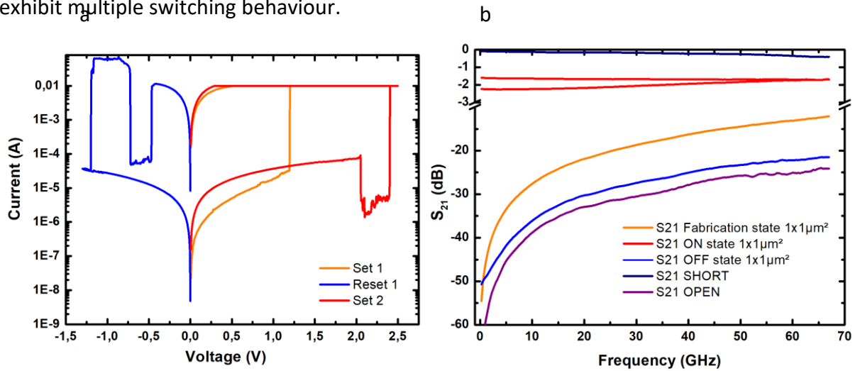
Figure 2 (a) I-V characteristics with multiple cycle on the same 1x1 \mu\text{m}^2 device with the interface Ni/MoS 2 /Ni. (b) S 21 parameter of a 1x1 \mu\text{m}^2 device with multiple switching cycle. The insertion loss is -1.5 dB at 67GHz and an isolation of -20 dB at 67 GHz for the OFF state of the device.
