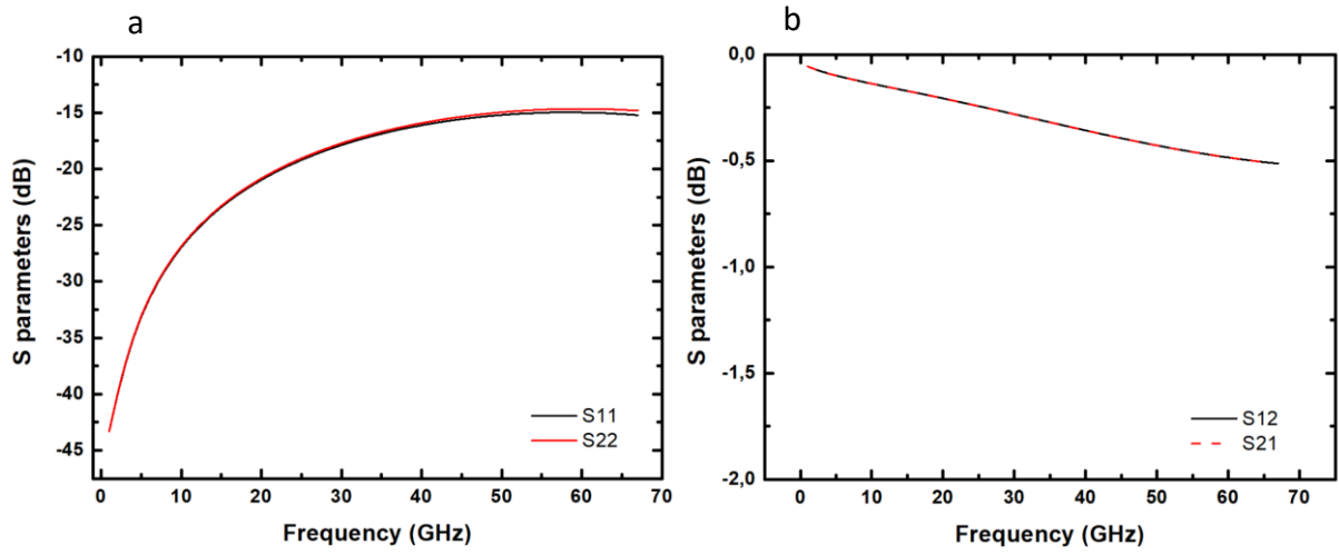
Figure 3 (a) Reflexion parameters S_{11} and S_{22} (b) transmission parameters S_{12} and S_{21} of the CPW. The S_{21} is -0.5 dB at 67 GHz (89.1% of the power transmitted). For the reflexion it reaches -15 dB at 67 GHz (3.16% of the power is reflected)
