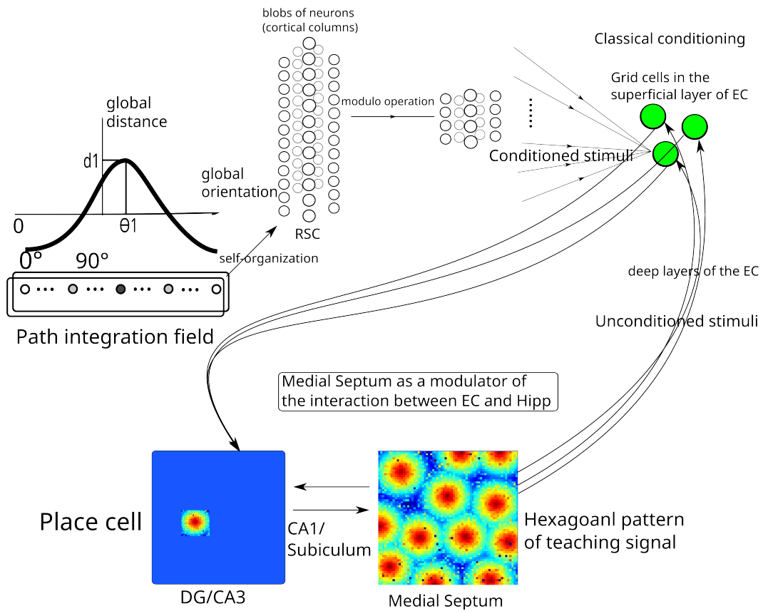
Figure 4.14: Model of the grid cell based on the reciprocal connection between the hippocampus and the entorhinal cortex.
