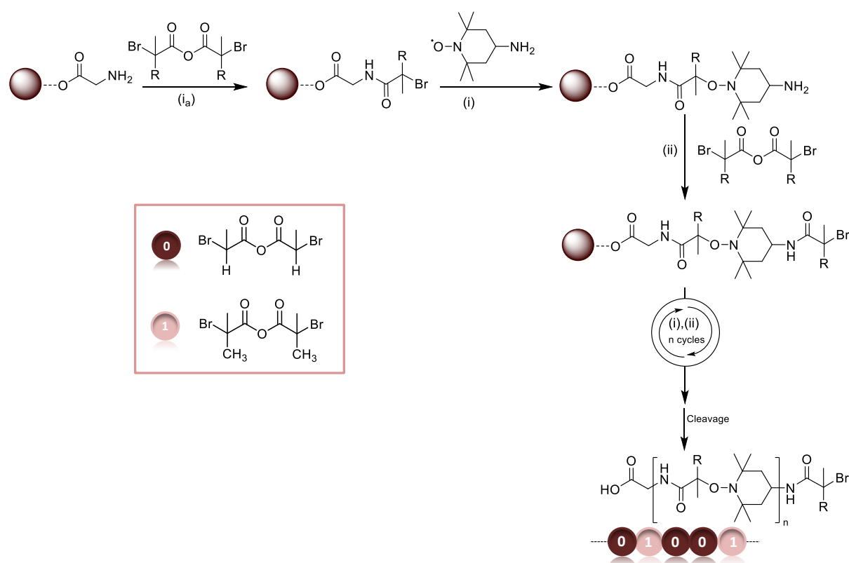
Figure I. 26: General strategy for the solid-phase synthesis of poly(alkoxyamine amide)s. Experimental Conditions: (ia) K 2 CO 3 for 1-bit or DIPEA for 0 bit, THF, RT; (i) CuBr, Me 6 TREN, DMSO or DMSO, microwaves at 40 °C and cleavage TFA, CH 2 Cl 2 .
