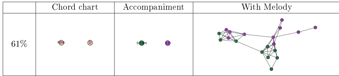
Figure 6.2.3: Comparison of the three levels of analysis for Something in the Way at a scale of 61%. We can observe at level 2 the clear separation between the two types of musical bars according to their accompaniment.
