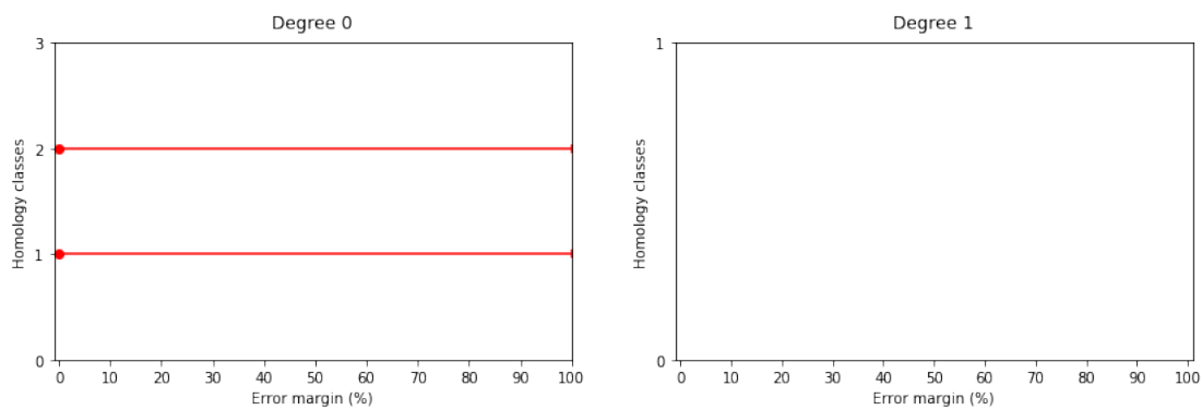
Figure 6.2.1: The associated family of barcodes for the harmonization of Something in the Way for levels 0 and 1 of analysis (the filtrations are the same in both cases).
