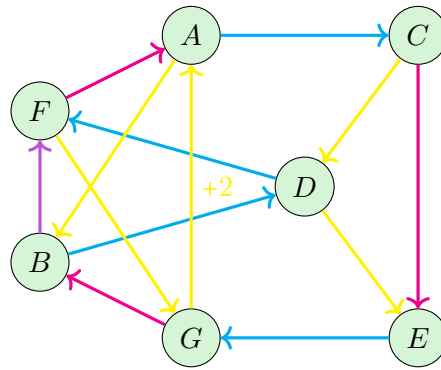
Figure 5.1.11: The associated filtration with the C -major scale at a scale of 98%. The new edges are given by the major seconds \{C, D\} , \{D, E\} , \{G, A\} and \{A, B\} , which provide a new one-dimensional cycle that lasts until 100% of the filtration.
